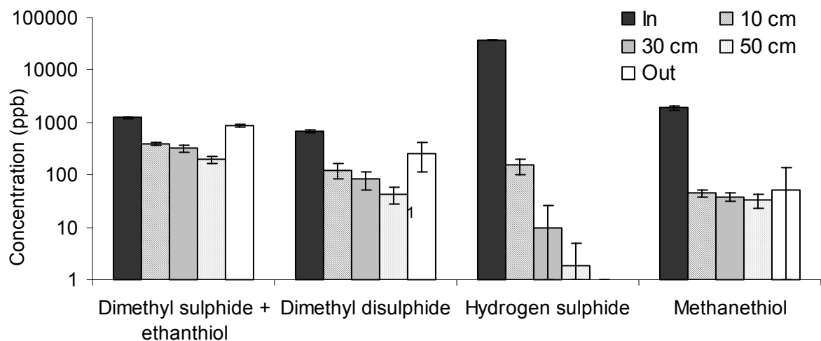
Fig. 4. Concentrations of selected compounds present in standard gas at increasing compost depth when passed through a column of MSW compost, with a bulk density of 740\text{kg/m}^3 , 50% moisture content, at 250\text{ml/min} for 96 minutes ( n = 3 , means \pm\text{SD} ).
