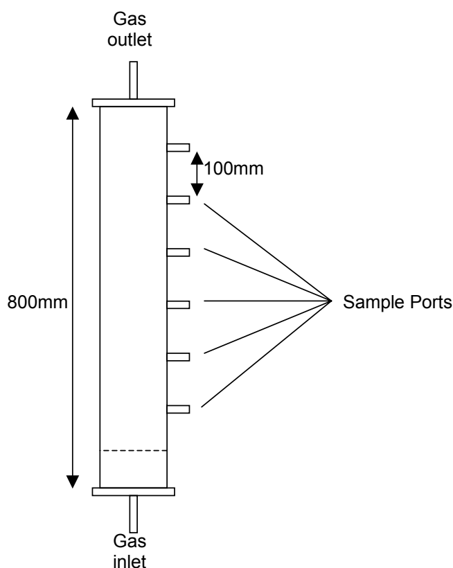
Fig. 1: Test rig used to assess effectiveness of compost as a daily cover material for odour reduction
