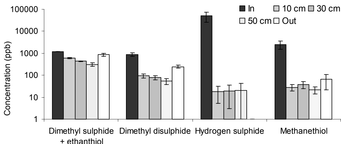
Fig. 3. Concentrations of selected compounds present in standard gas at increasing compost depth when passed through a column of MSW compost, with a bulk density of 590kg/m 3 , 35% moisture content, at 250ml/min for 96 minutes ( n = 3 , means \pm SD).
