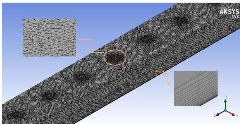
Fig. 3. Schematic view of the computation mesh
