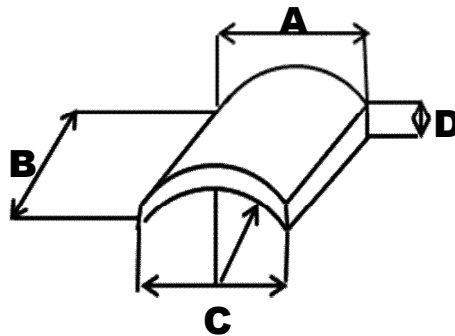
Figure 1 Sample geometry used in this work for fireside corrosion test A – chord length, B – length of the sample, C – arc and D – wall thickness
