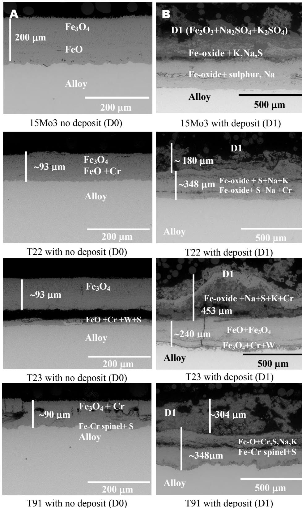
Figure 5 BSE images of materials exposed in simulated oxy-fired combustion gases at 600 °C for 1000 hours; column (A) materials without any deposit (D0), (B) materials with deposit (D1)
