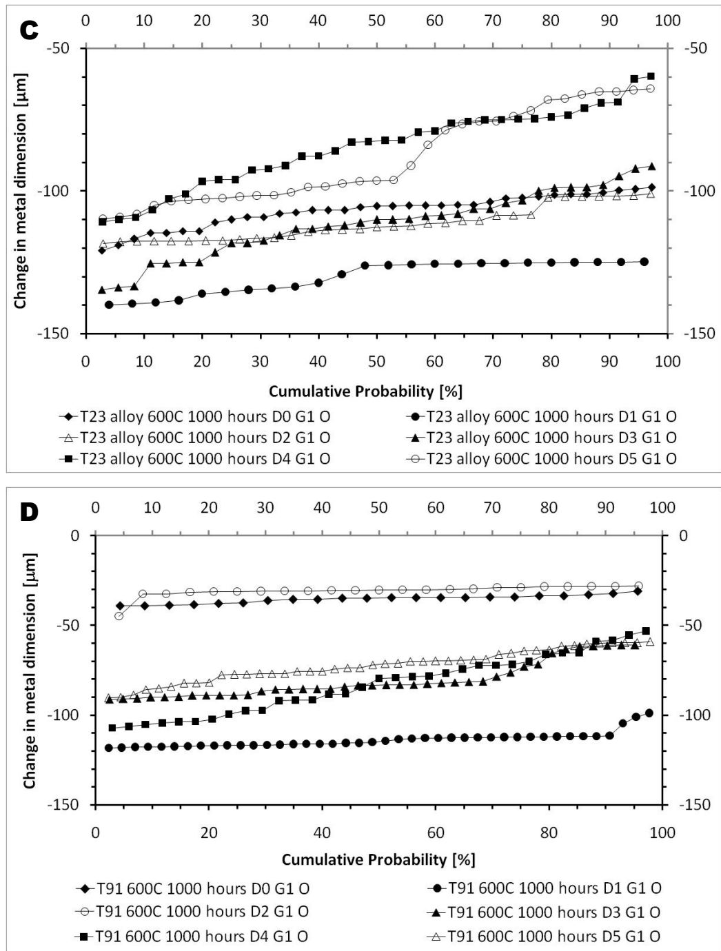
Figure 6 Dimensional metrology of the samples exposed at 600 °C, A 15Mo3, B) T22, C) T23 and D) T91
