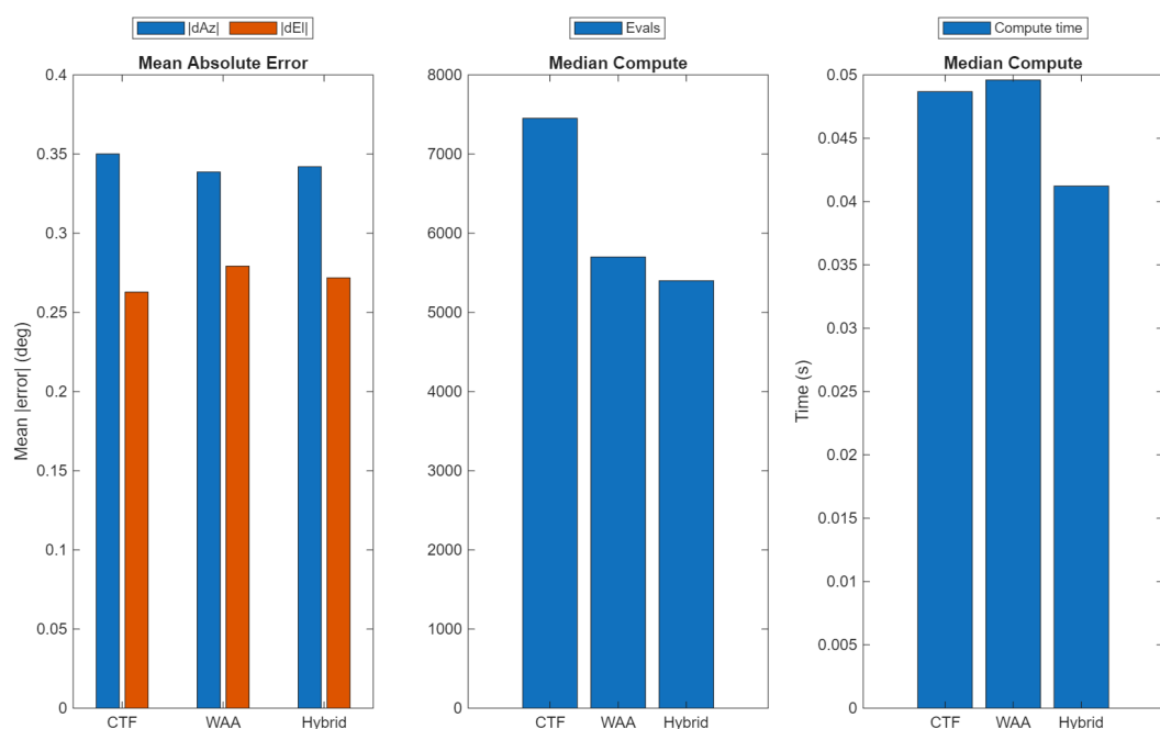
Figure 12. Aggregate comparison over the 10 cases at 15 m/s: mean absolute errors (left), median compute statistics (center) and runtime (right).
