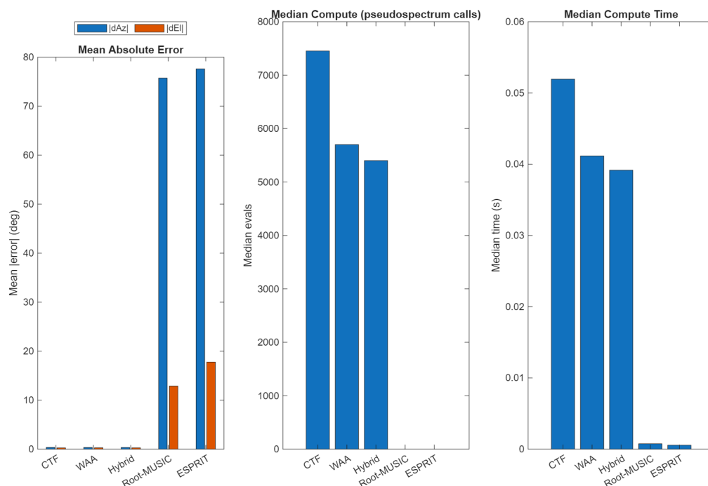
Figure A1. Pose-Aware MUSIC comparison with root-MUSIC and ESPRIT.
