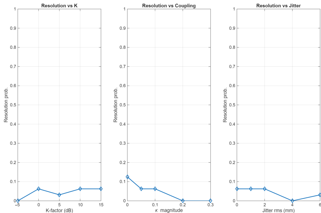
Figure 15. Resolution probability for two equal-power sources 8^\circ apart in azimuth versus K , \kappa , and jitter, all derived from FEKO-based platform characterizations.
