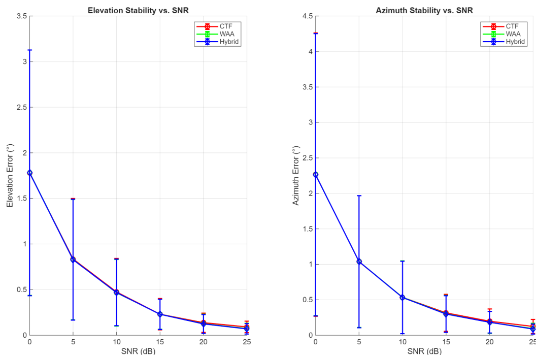
Figure 11. Stability vs. SNR (mean \pm std of absolute error over 10 cases). (Left): elevation; (right): azimuth.
