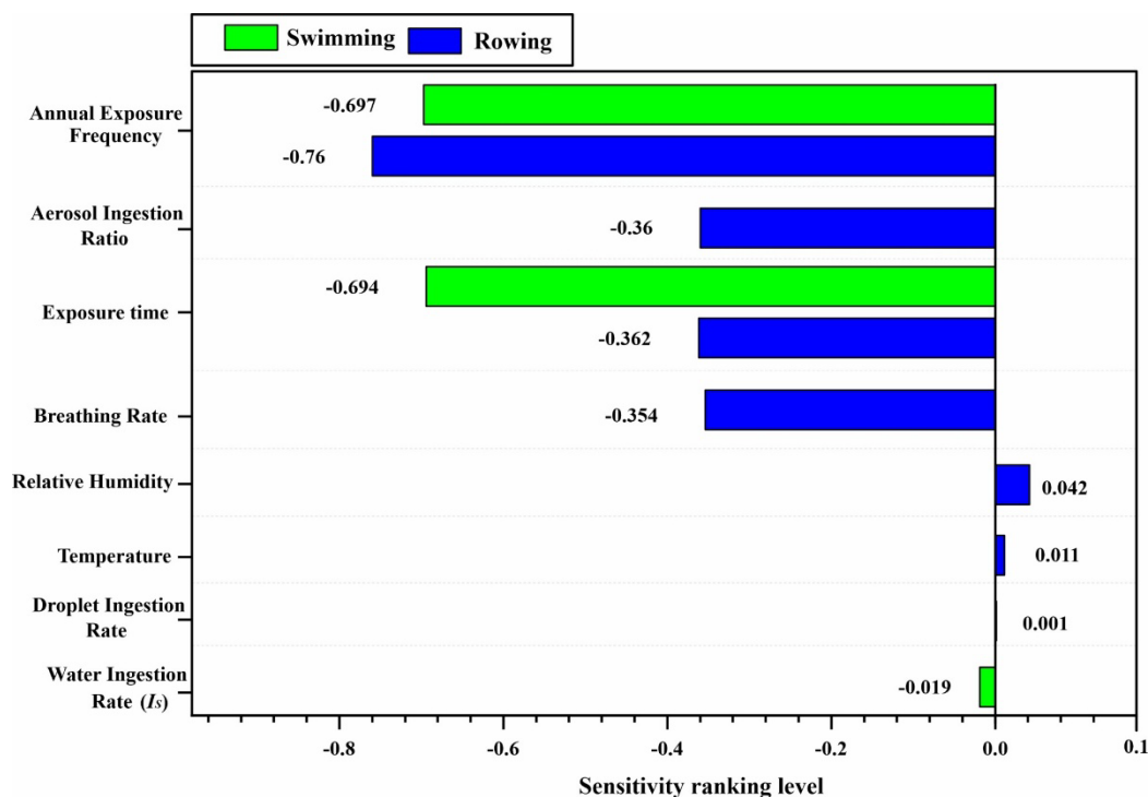
Fig. 3 Sensitivity analysis based on the ranking of input variable parameters that affect the TLVs of acceptable exposure concentration when nearby residents are rowing and swimming.
