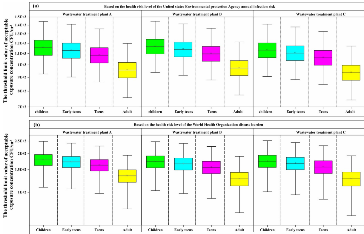
Fig. 1 Threshold limit values (TLVs) of acceptable E. coli exposure concentrations (CFU/m 3 ) for residents engaged in rowing, based on discharges from WWTPs A, B, and C. (a) U.S. EPA annual infection risk; (b) WHO disease burden benchmark. The simulation was run for 10,000 iterations; the bottom and top of the box represent the first and third quartiles (25th and 75th percentile values, respectively). The band inside the box represents the second quartile (median), and the tetragon denotes the average. The bottom and top of the whiskers represent the 5th (optimistic estimate in the best-case scenario) and 95th (conservative estimate in the worst-case scenario) percentiles, respectively.
