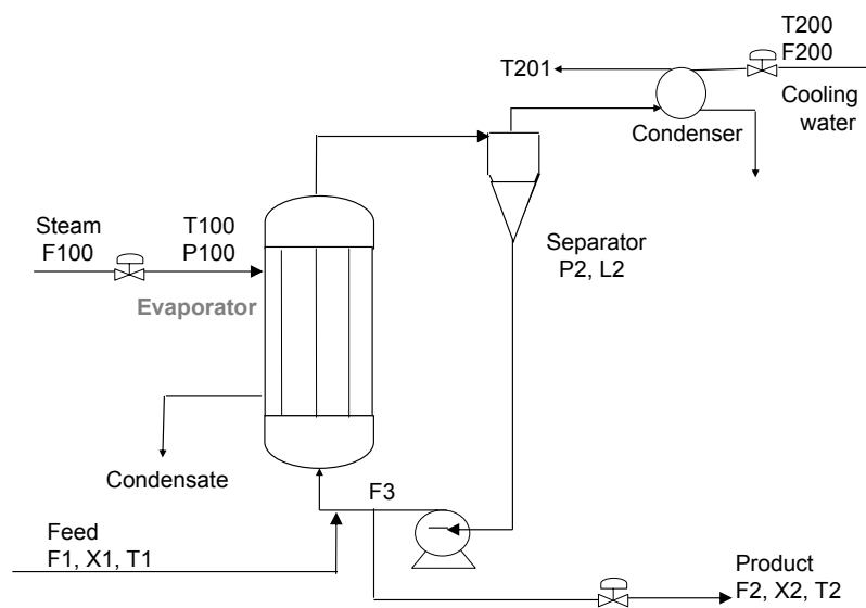
Figure 1: Evaporator System
