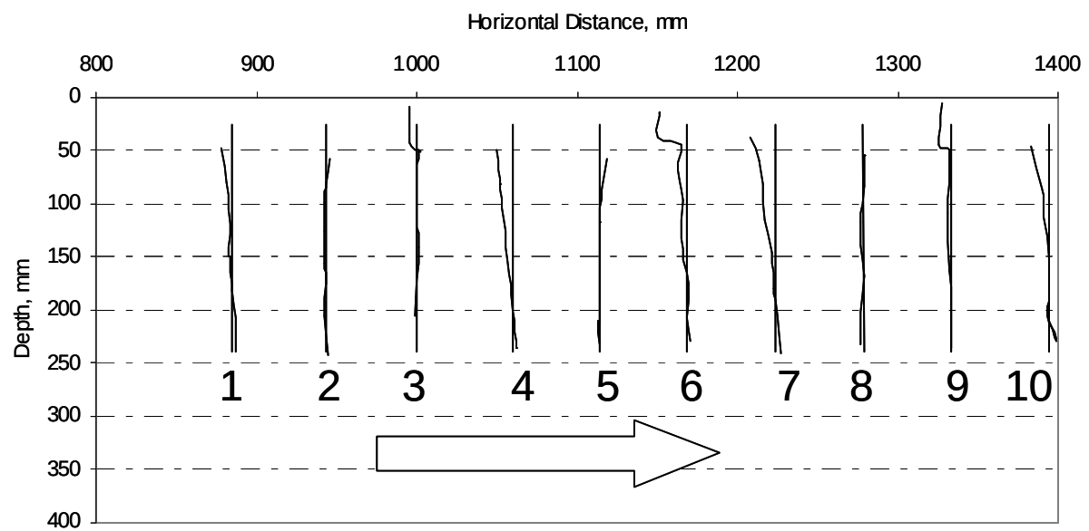
Figure 12. A digital image of the longitudinal position of the sand columns after the passage of a 12 t rubber track
