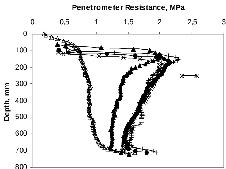
Figure 5. Penetrometer resistance for different undercarriage systems. Tracked undercarriages Group a) \Delta , Control; \square , Track+700mm/4.5t/1.0bar; \blacksquare , Track+500-70mm/4.5t/2.3bar. Wheeled Undercarriages Group b) \Delta , Control; \times , 900mm/10.5t/1.9bar+500-70mm/4.5t/2.3bar; + , 900mm/10.5t/1.9bar+700mm/4.5t/1.0bar; \bullet , 680mm/10.5t/1.9bar+500-85mm/4.5t/1.4bar; \blacktriangle , 900mm/5t/0.5bar three passages; *, LSD at 95% confidence level
