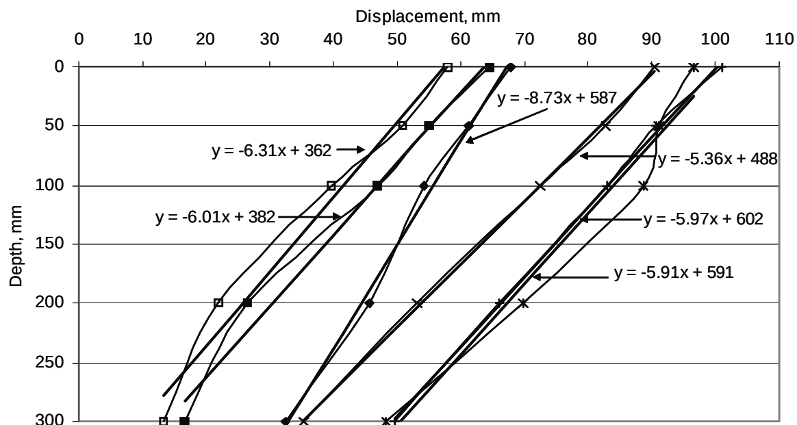
Figure 9. Displacement vs. Depth, top 300 mm with regression lines. \square , track 10.5t; \blacksquare , track 12t; * , 680mm/10.5t/2.2bar; \times , 900mm/10.5t/1.9bar; + , 800mm/10.5t/2.5bar; \blacklozenge , 800mm/10.5t/1.25bar;
