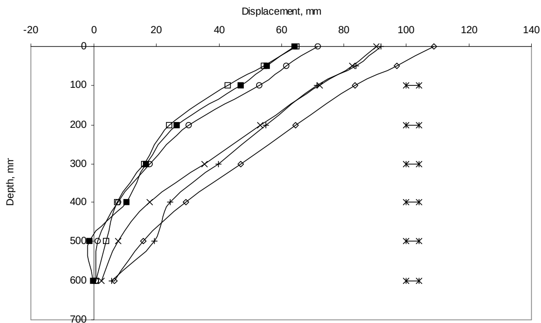
Figure 2. Soil displacement caused by the front axle and additional soil displacement caused by the rear axle. ■, Track alone; □, Track+700mm/4.5t/1.0bar; ○, Track+500-70mm/4.5t/2.3bar; ×, 900mm/10.5t/1.9bar alone; +, 900mm/10.5t/1.9bar + 700mm/4.5t/1.0bar; ◇, 900mm/10.5t/1.9bar + 500-70mm/4.5t/2.3bar; *, LSD at 95% confidence level
