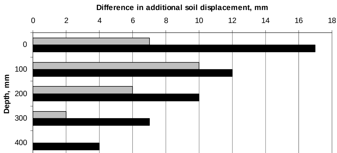
Figure 3. Difference in additional soil displacement from 500-70mm/4.5t/2.3bar compared to 700mm/4.5t/1.0bar following both a leading track (grey) or a tyre (black)
