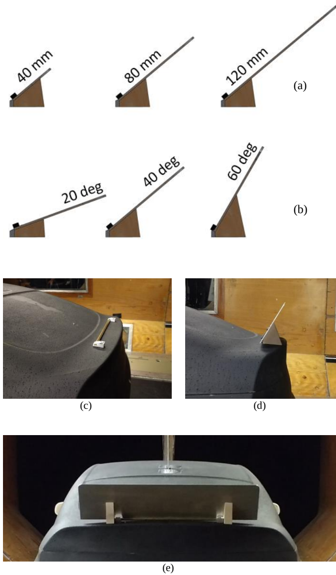
Figure 7. Rear-end Spoiler. CAD illustration of (a) size and (b) angles of incidence; (c) common spoiler mounting; (d) fitting a spoiler plate and block supports; (e) sample of a spoiler case ready for experimental test.
