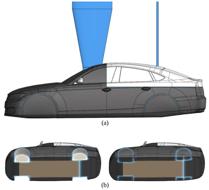
Figure 3. CAD sample of the Cranfield modified version of the DrivAer body with smooth underfloor: (a) baseline car case as experimentally tested (FS*wMwoW, GS on, wTS), (b) highlight on the modified edges: extension of the main underfloor surface, wheel cavities (wW) and wheel lids (woW).
