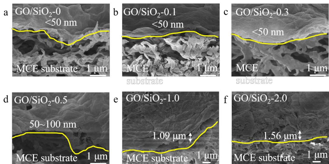
Figure S7. Cross-sectional SEM images of GO/SiO 2 -x (x=0, 0.1, 0.3, 0.5, 1.0, 2.0 corresponding to a, b, c, d, e, f) membranes prepared by using 0.5 ml GO/SiO 2 -x dispersions.
