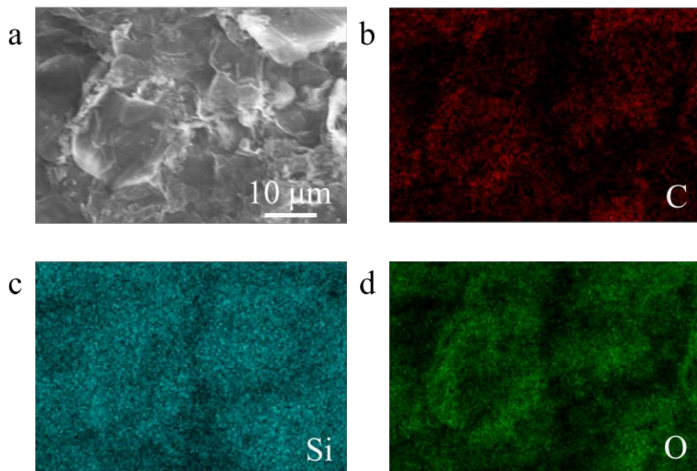
Figure S8. Surface elemental mapping images of the GO/SiO 2 -2.0 membrane. (a) Surface SEM image of the GO membrane. (b) Elemental mapping of C on the GO/SiO 2 -2.0 membrane. (c) Elemental mapping of Si on the GO/SiO 2 -2.0 membrane. (d) Elemental mapping of O on the GO/SiO 2 -2.0 membrane.
