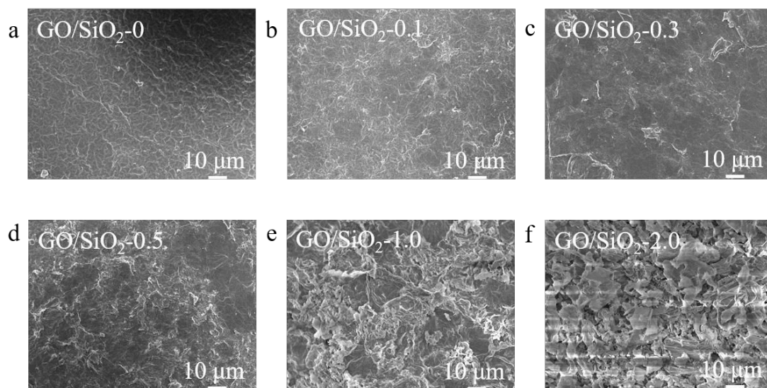
Figure S6. Surface SEM images of GO/SiO 2 -x (x=0, 0.1, 0.3, 0.5, 1.0, 2.0 corresponding to a, b, c, d, e, f) membranes.
