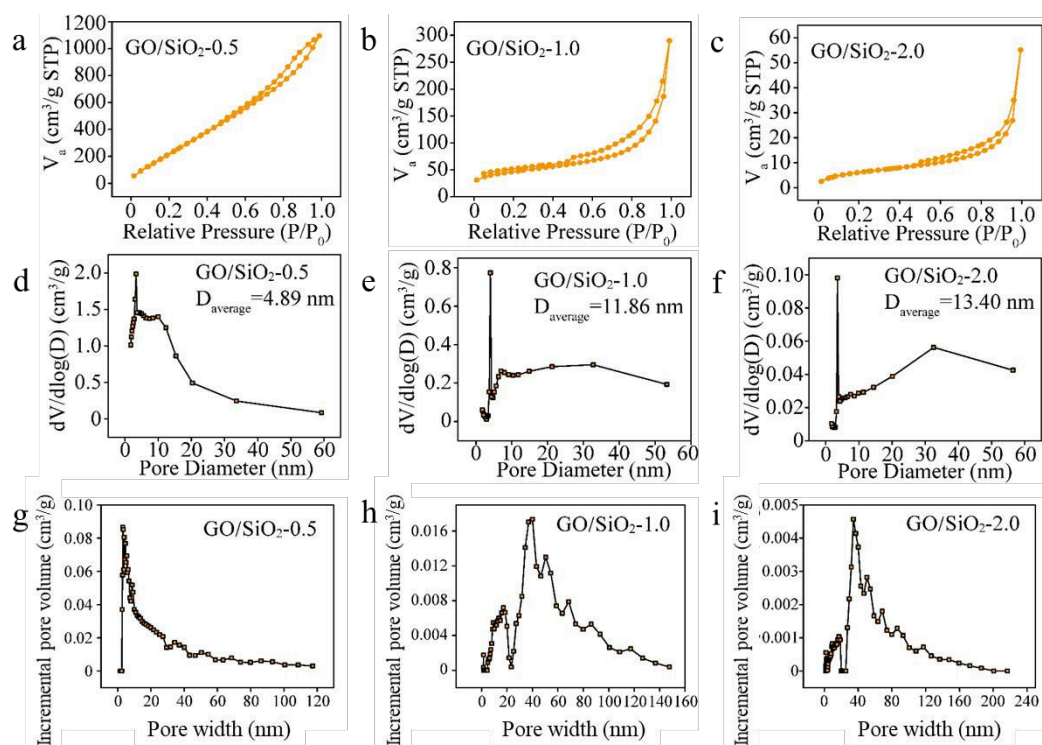
Figure S9. Results of Brunauer-Emmett-Teller (BET) surface area measurements for \text{GO/SiO}_2-x membranes. (a-c) \text{N}_2 adsorption-desorption isotherm of \text{GO/SiO}_2-0.5 , 1.0 and 2.0 membranes. (d-f) Pore diameters test of \text{GO/SiO}_2-0.5 , 1.0 and 2.0 membranes, the average pore diameters of \text{GO/SiO}_2-0.5 , 1.0 and 2.0 membranes are 4.89 \text{ nm} , 11.86 \text{ nm} and 13.40 \text{ nm} . (g-i) Incremental pore volume of corresponding pore width in \text{GO/SiO}_2-0.5 , 1.0 and 2.0 membranes.
