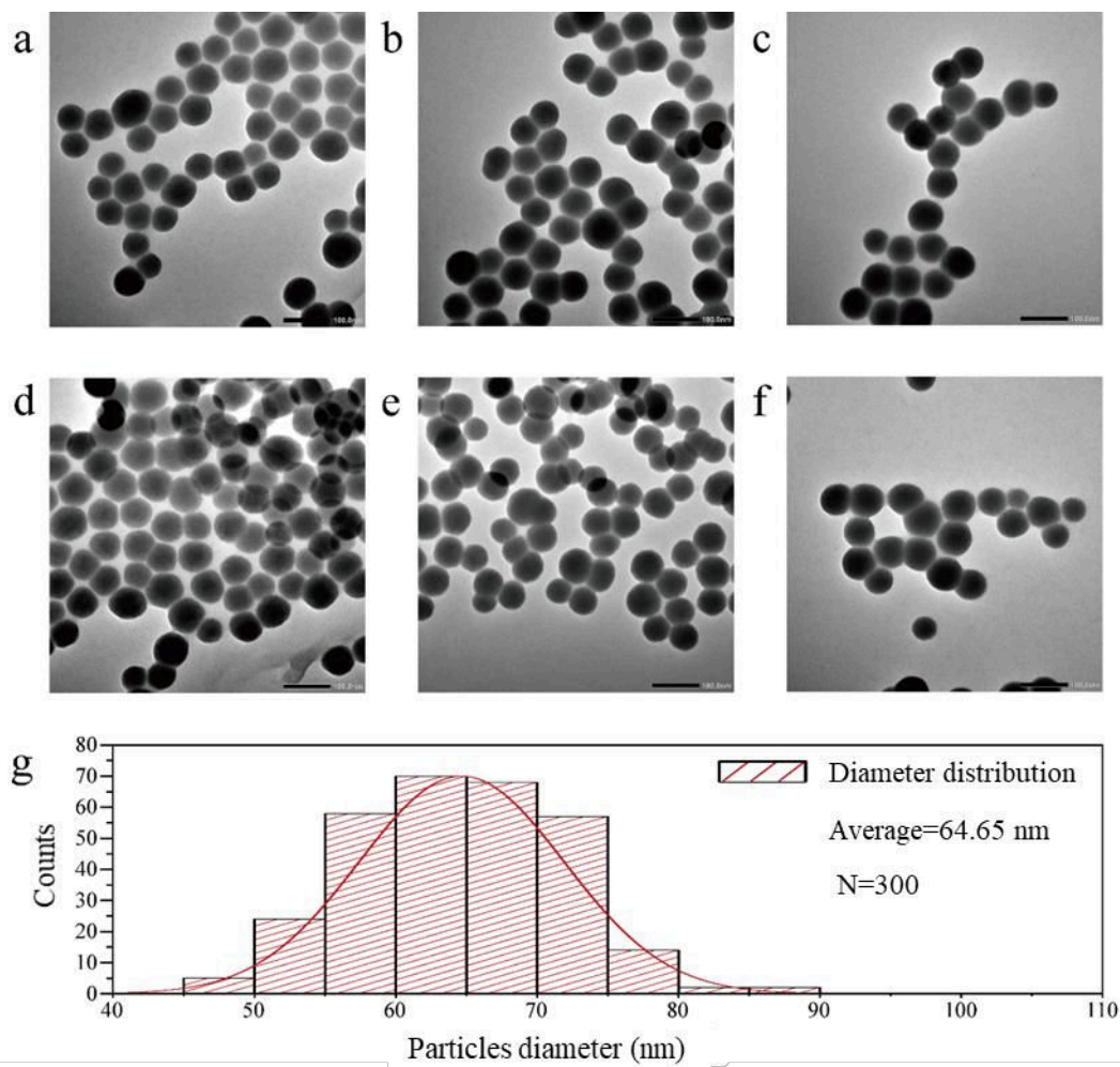
Figure S12. (a-f) TEM images of \text{SiO}_2 nanoparticles in \text{SiO}_2 -2.0 colloids. (g) Diameter distribution of \text{SiO}_2 nanoparticles computed according to S12a-f.
