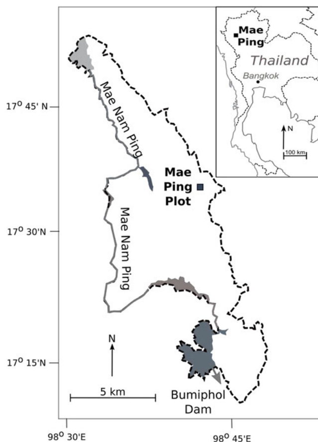
Figure 1. Location of Mae Ping Forest Ecology plot: Dashed line – Mae Ping National Park boundary Shaded – Mae Ping river, Bhumibol Dam, & other lakes; Solid square – Mae Ping Forest Ecology Plot.
