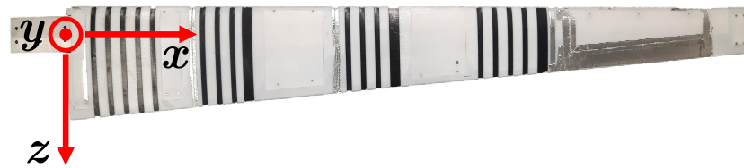
Figure 2. XB-2 wing top view. Y-axis coming out of the page. Any apparent distortions are due to lens-induced optical effects. (Adapted from [28]).
