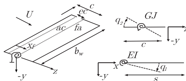
Figure 3. Flexible wing 2 DoF model schematic.
