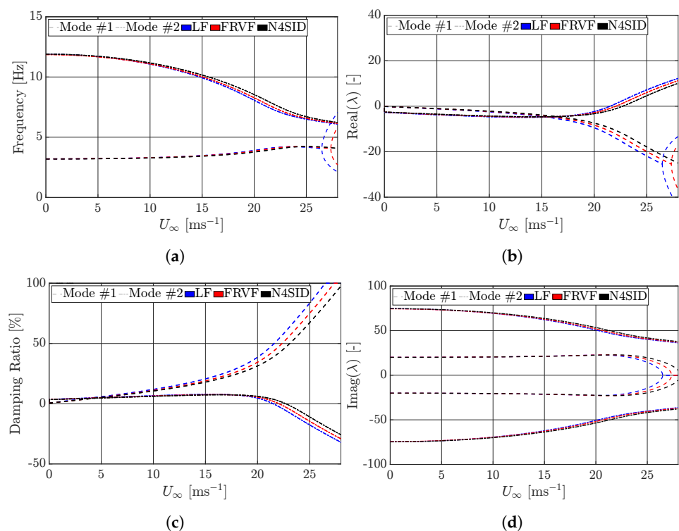
Figure 4. XB-2: Frequency (a), damping ratio (c), real (b), and imaginary part (d) of the eigenvalues vs. U_\infty plots for the aeroelastic model computed from data obtained via LF, FRVF, and N4SID for the baseline scenario.
