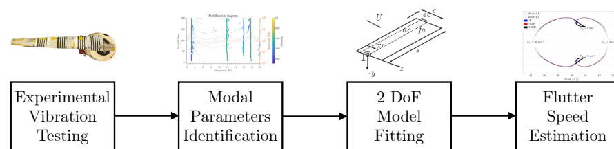
Figure 1. Flutter speed estimation workflow.
