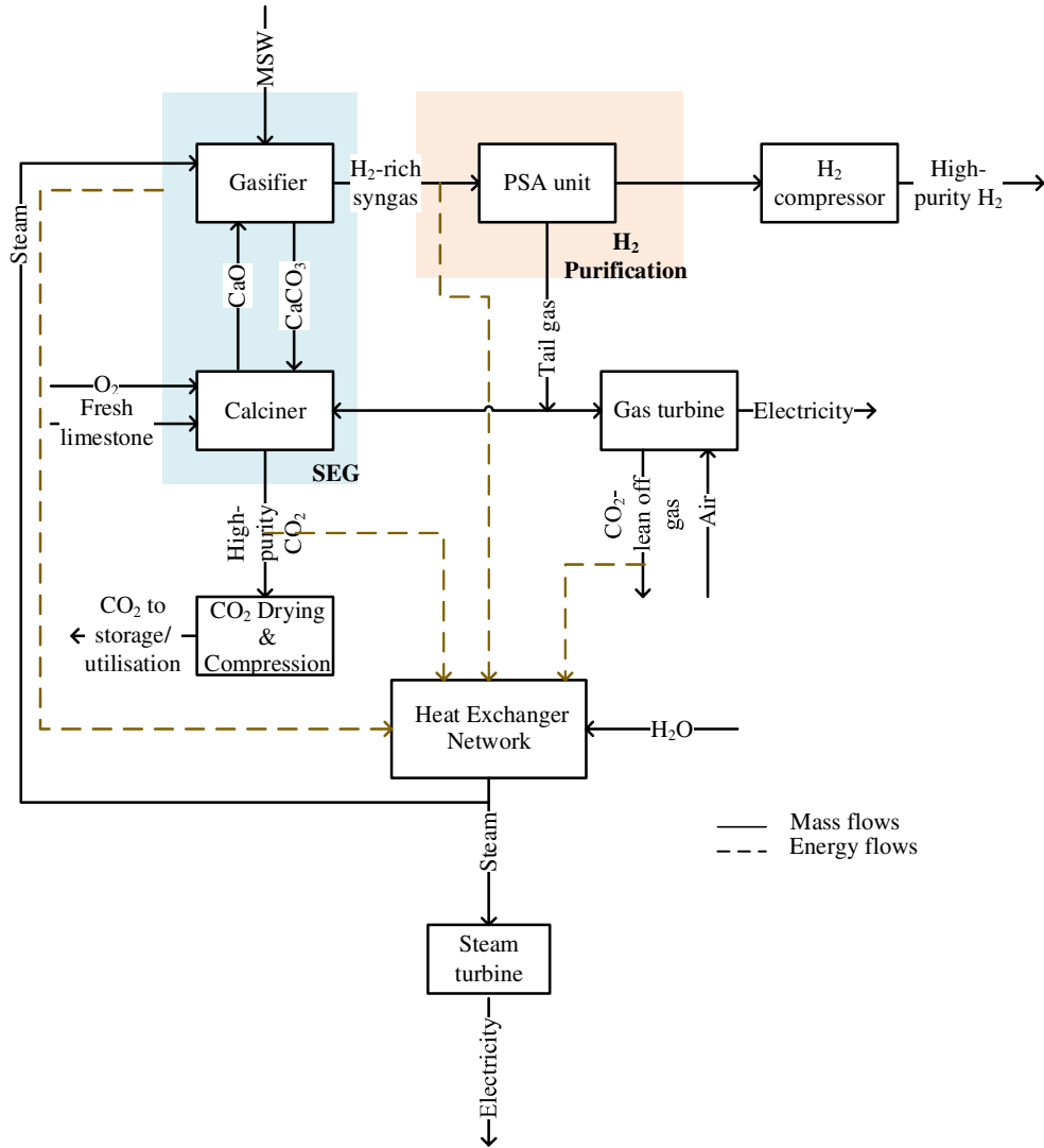
Figure 3. Simplified diagram of municipal solid waste sorption enhanced gasification for hydrogen production
