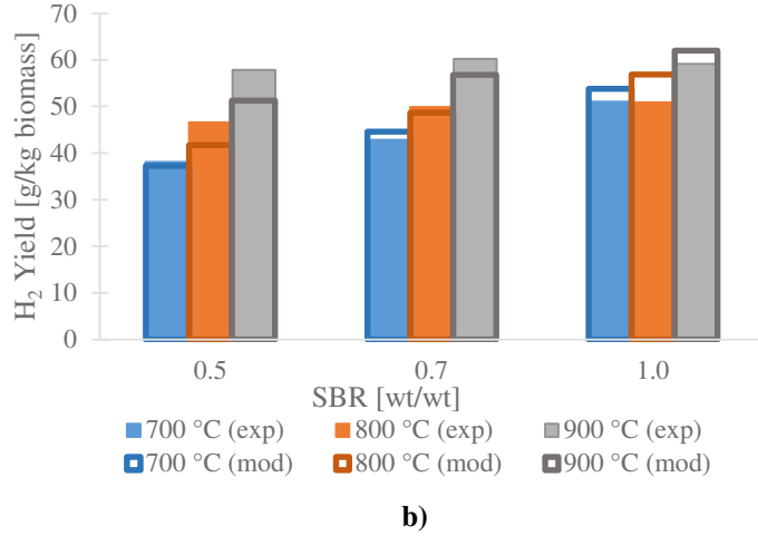
Figure 2. Validation of the municipal solid waste steam gasification model with experimental data, obtained at three different temperatures and steam-to-biomass ratios, in terms of a) gas composition and b) hydrogen yield. Exp and mod correspond to experimental and simulated data, respectively. [10]
