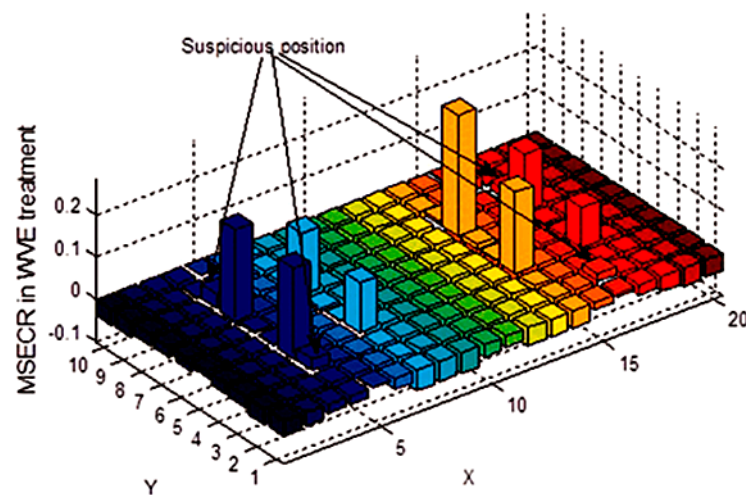
Figure 9. Enhanced modal strain energy change ratio (MSECR) method localization of multiple defects in a two-span plate with 2% noise [189].
