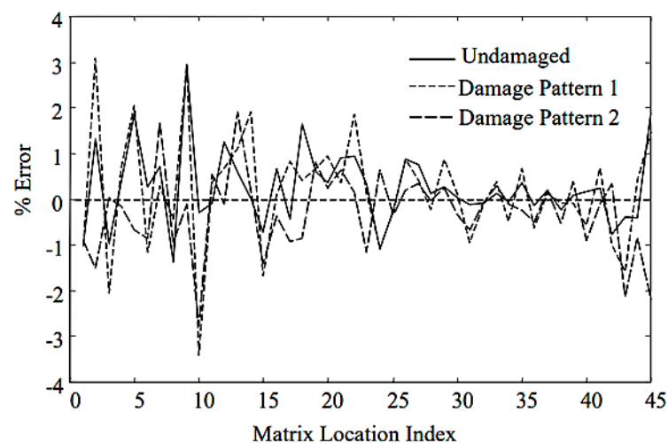
Figure 10. Damage location vector (DLV) method error [237].
