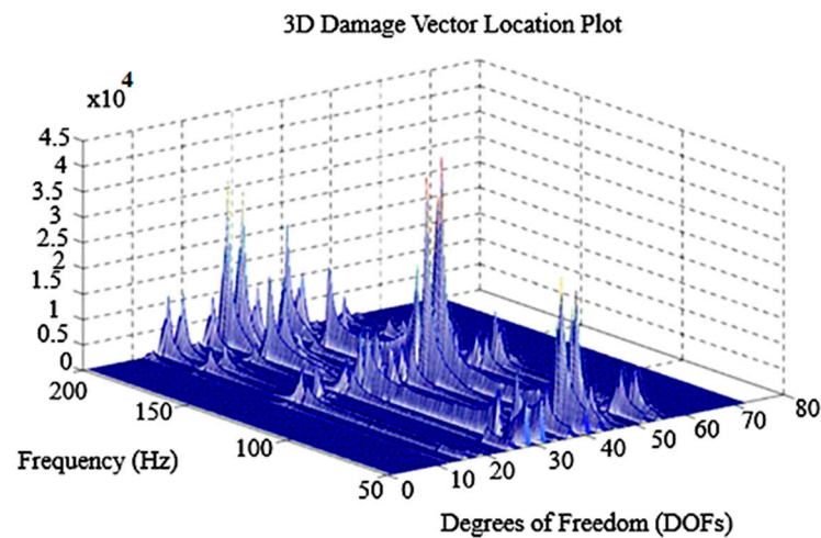
Figure 8. Damage detection in element 11 by the damage location vector method [183].
