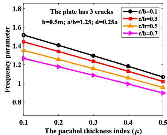
Figure 4. The correlation between the frequency parameter and the index of parabolic varying thickness (PVT) contains 3 cracks, where (c) crack length, (d) distance between cracks, and (a and b) plate length and width, respectively [167].
