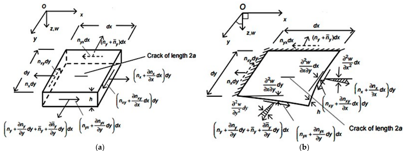
Figure 1. (a) In-plane forces acting on the plate, and (b) cracked plate deformation and two-sided constraints [83].
