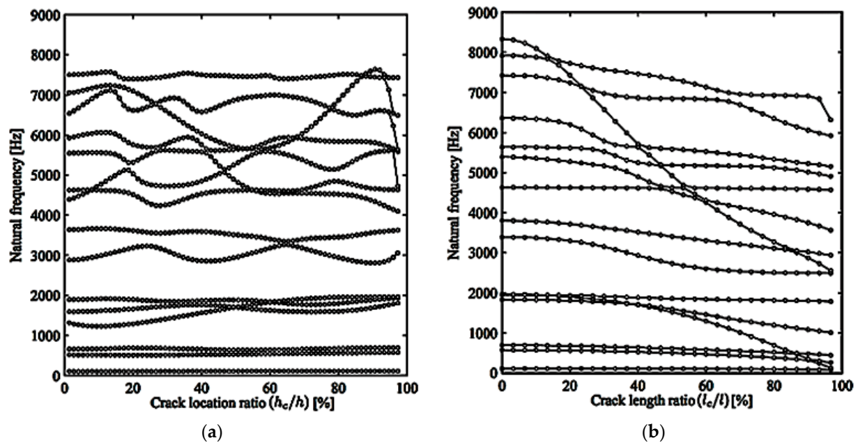
Figure 2. Variation of the first 15 natural frequencies with respect to crack (a) location ratio and (b) length ratio [99].
