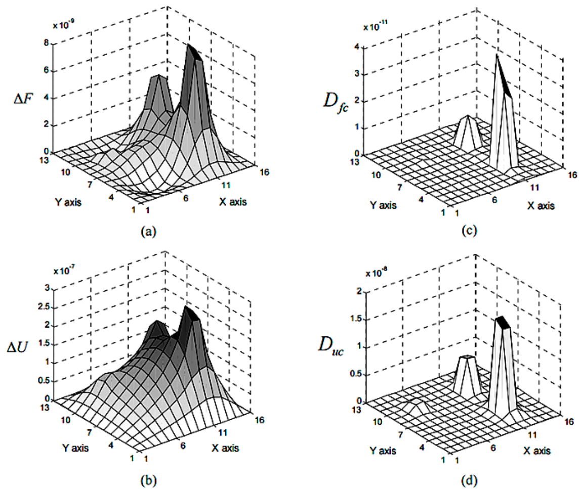
Figure 6. Comparison between different methods for locating damage based on changes in the modal flexibility: (a) index of flexibility change; (b) index of uniform load surface (ULS) change; (c) index of flexibility curvature; (d) index of ULS curvature [174].
