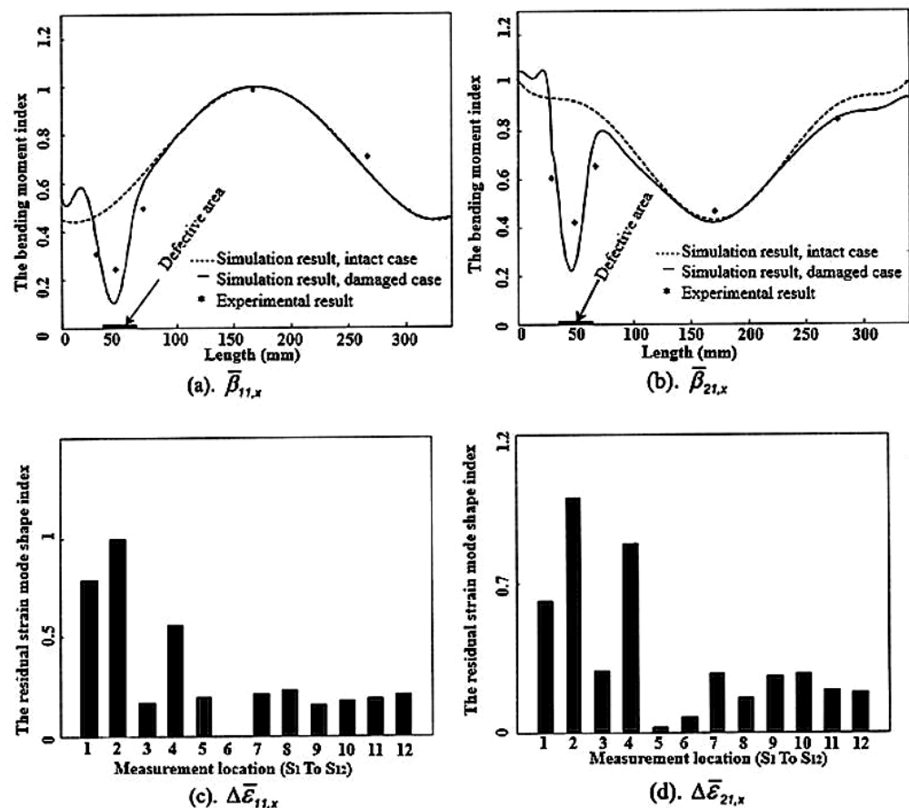
Figure 5. The bending moment index ( \bar{\beta}_{r,x} ) results for (a) modes (1,1) and (b) mode (2,1), along with the residual strain mode shape index ( \Delta \bar{\epsilon}_{r,x} ) results for (c) modes (1,1) and (d) mode (2,1) [173].
