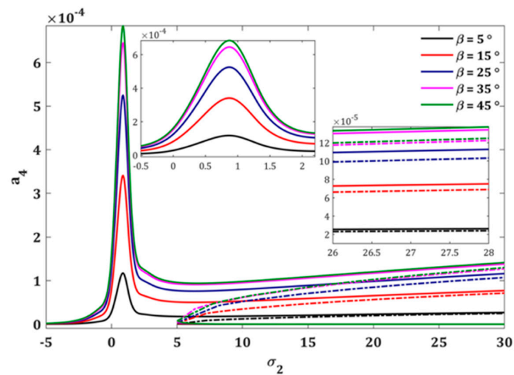
Figure 3. Frequency response curve at different crack angles, where a_4 is the peak amplitude at mode 4, and \sigma_2 is the second perturbation parameter [132].
