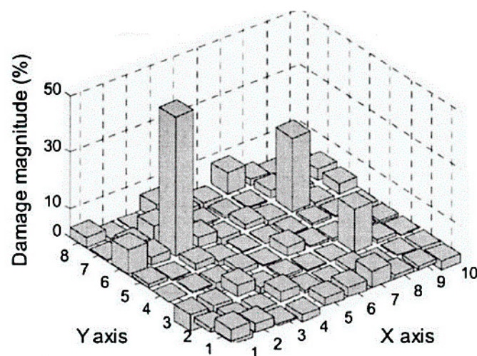
Figure 7. Damage magnitude percentage for the two-dimensional cracked plate [178].
