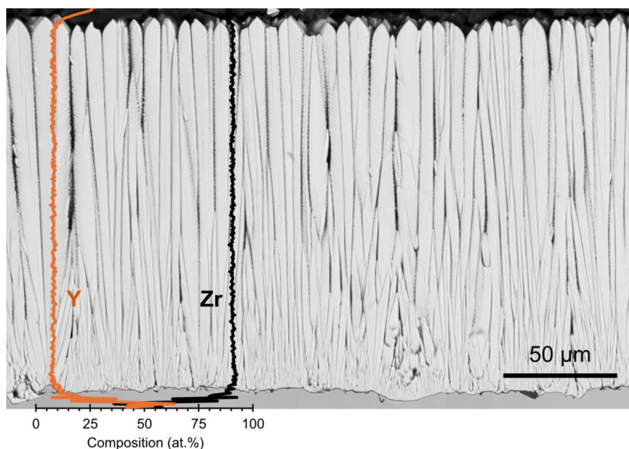
Fig. 3. Cross-section of PYSZ TBC on aluminised Nimonic 75 alloy in as-deposited condition taken with backscattered detector, overlaid with EDX linescan normalised to only include the metallic elements of the oxides (Y in orange and Zr in black).
