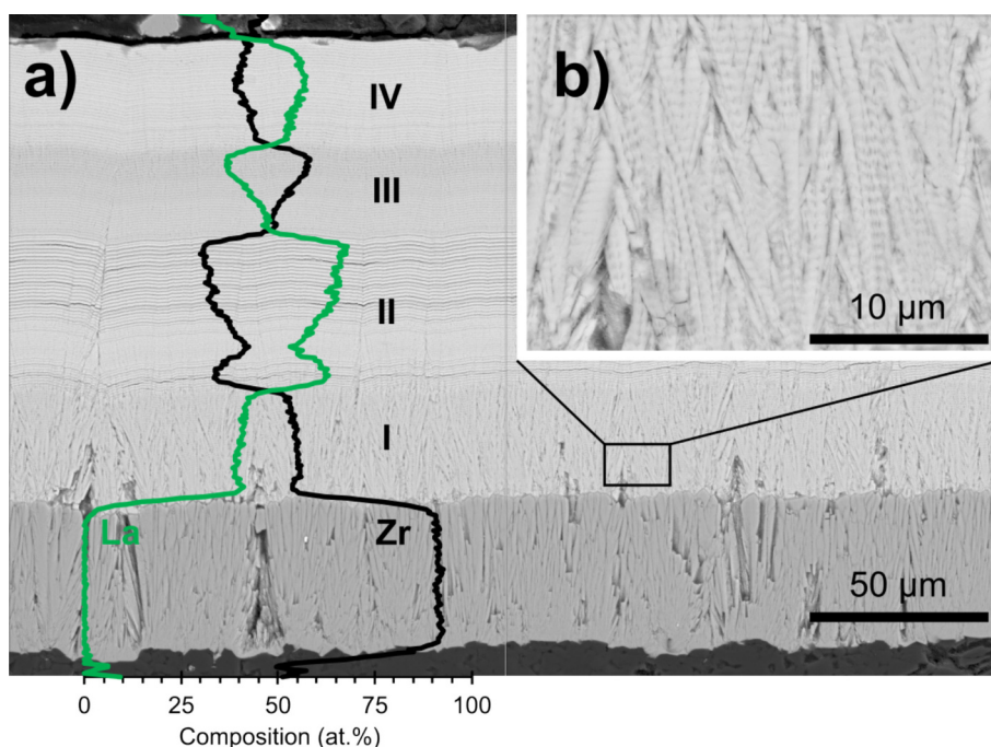
Fig. 7. Cross-section of lanthanum zirconate TBC on alumina, co-evaporated from LZ and PYSZ ingots, a) in as-deposited condition taken with backscattered detector overlaid with EDX linescan normalised to only include the metallic elements of the oxides (La in green, Zr in black, Y not plotted), presents four distinct Regions I-IV. b) Higher magnification of the lower region (I).
