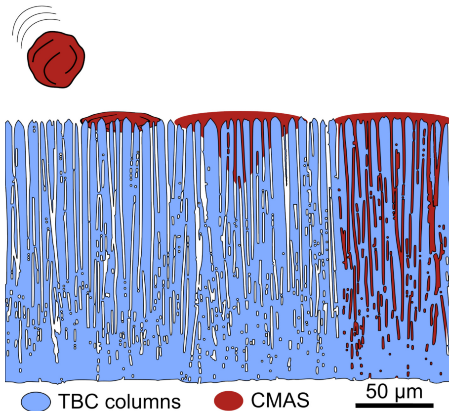
Fig. 1. Diagram of CMAS infiltration on a TBC deposited by EB-PVD. From left to right, the CMAS particles approach the coating, impact, melt, and infiltrate down the columnar interspace.
