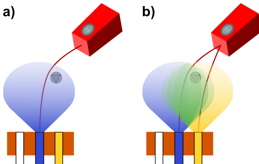
Fig. 2. Comparison of the distributions of the evaporation plumes of a) single-ingot evaporation and b) co-evaporation of two ingots, illustrated by different ingot colours.
