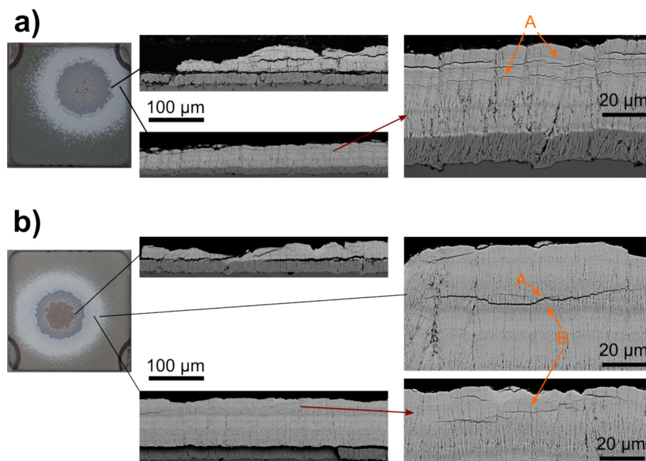
Fig. 14. Composite images of eroded LZ TBC samples. The macroscopic optical image indicates the locations where cross-sections were taken with backscattered SEM detector. a) is the lowest performing sample where extensive cracks appear located in composition bands, b) is the best performing LZ but extensive cracking is also noticeable.
