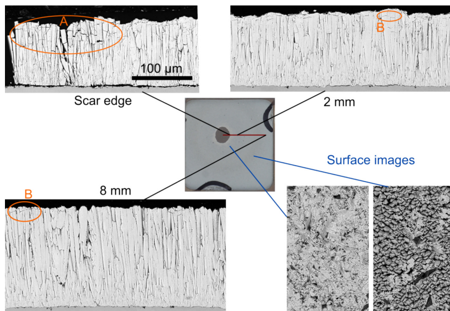
Fig. 11. Composite image of an eroded PYSZ TBC sample. The macroscopic optical image indicates the locations where cross-sections and surface images were taken with backscattered SEM detector (all at the same magnification). The reference positions of the cross-sections are related to the distance to the edge of the delaminated area (scar).
