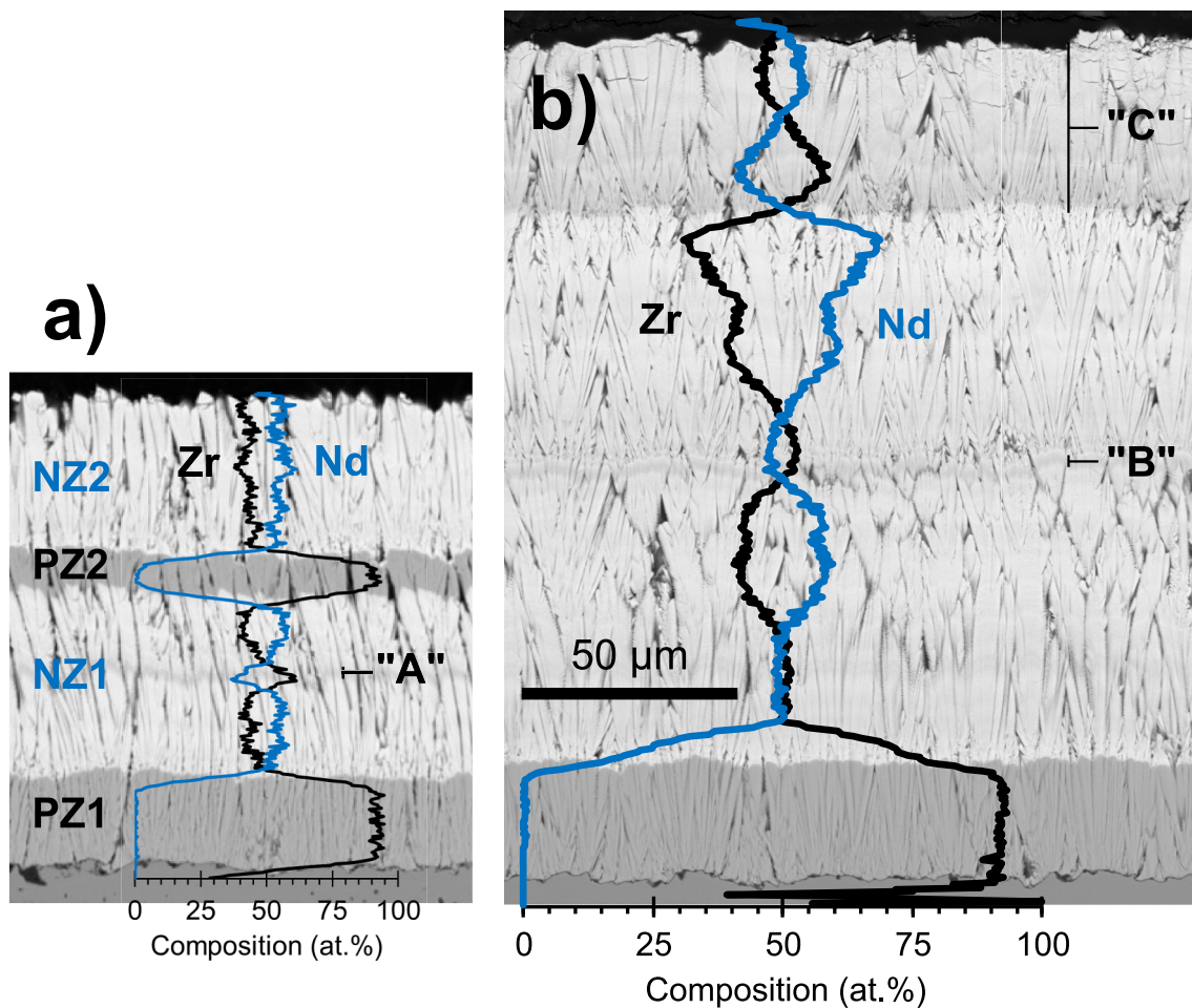
Fig. 5. Cross-section of neodymium zirconate TBC on aluminised Nimonic 75 alloy in as-deposited condition taken with backscattered detector, a) from 4-layer system and b) from 2-layer coating overlaid with EDX linescan normalised to only include the metallic elements of the oxides (Nd in blue, Zr in black, Y not plotted). Key regions have been highlighted and named by capital letters.
