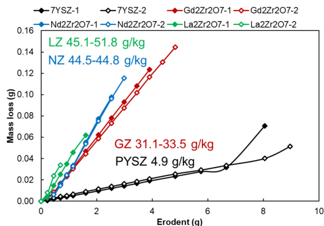
Fig. 10. Curves of mass loss vs erodent used during erosion testing of PYSZ, GZ, NZ and LZ coatings including their steady state erosion rate.
