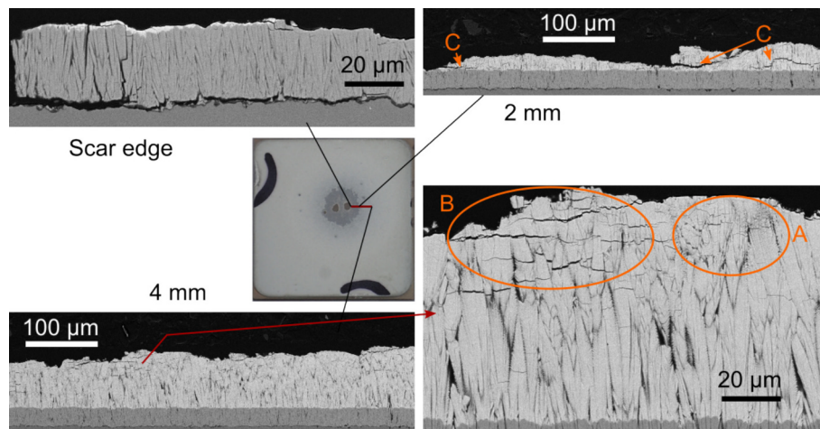
Fig. 12. Composite image of an eroded GZ TBC sample. The macroscopic optical image indicates the locations where cross-sections were taken with backscattered SEM detector. The reference positions of the cross-sections are related to the distance to the edge of the delaminated area (scar).
