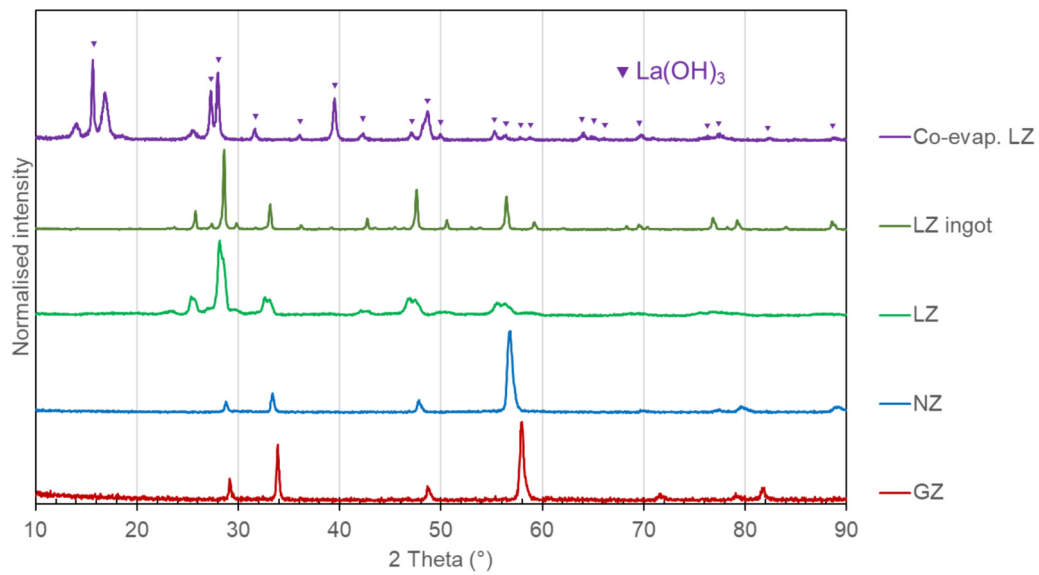
Fig. 8. XRD spectra obtained from the surface of co-evaporated LZ TBC, the LZ TBC produced from a single ingot, the LZ ingot, the NZ TBC and the GZ TBC.
