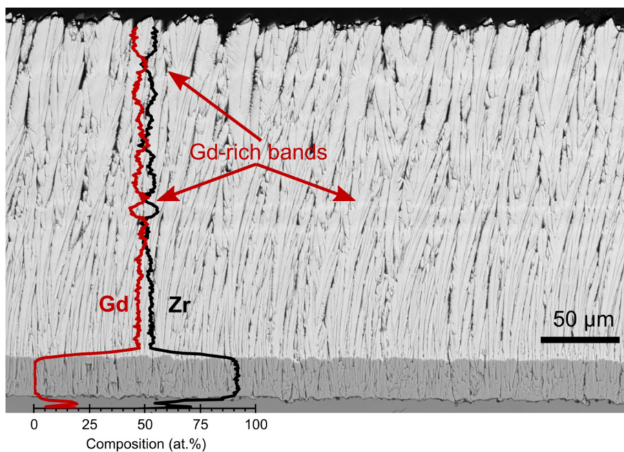
Fig. 4. Cross-section of gadolinium zirconate TBC on aluminised Nimonic 75 alloy in as-deposited condition taken with backscattered detector, overlaid with EDX linescan normalised to only include the metallic elements of the oxides (Gd in red, Zr in black, Y not plotted). Some Gd-rich banding is noticeable.
