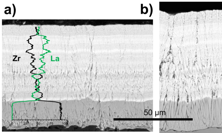
Fig. 6. Cross-section of lanthanum zirconate TBC in as-deposited condition taken with backscattered detector, a) on alumina substrate plus overlay of EDX linescan normalised to only include the metallic elements of the oxides (La in green, Zr in black, Y not plotted), and b) on aluminised Nimonic 75 alloy.
