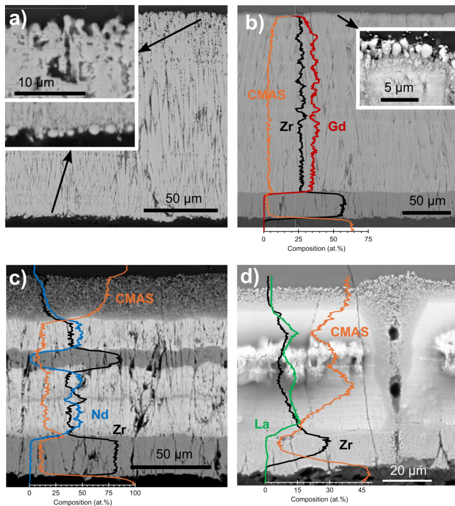
Fig. 9. Cross-section images of different TBCs after CMAS exposure for 30 min at 1300 °C taken with backscattered detector, overlaid with EDX linescan normalised to only include the metallic elements of the oxides. a) PYSZ, b) gadolinium zirconate, c) neodymium zirconate, d) lanthanum zirconate.
