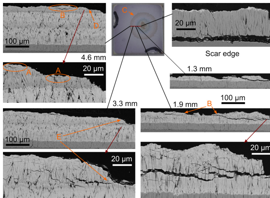
Fig. 13. Composite image of an eroded NZ TBC sample. The macroscopic optical image indicates the locations where cross-sections were taken with backscattered SEM detector. The reference positions of the cross-sections are related to the distance to the edge of the delaminated area (scar).
