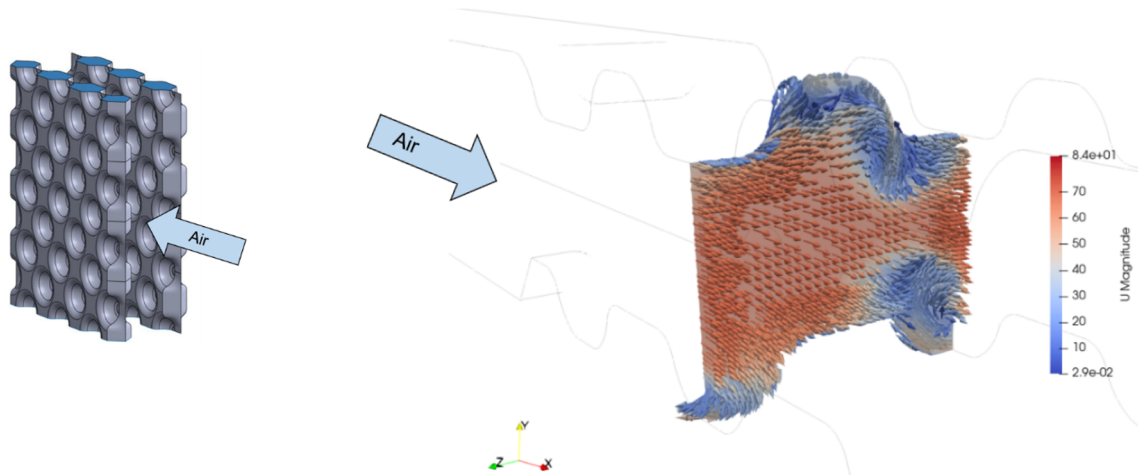
Fig. 5. Velocity field in HE cross-section [m/s] – Inlet velocity: 30 m/s.
