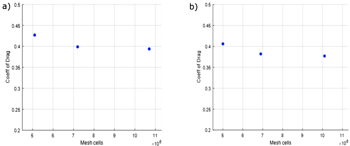
Fig. 15. Mesh independence study on C_D : a) 'base' case b) 'new' case.
