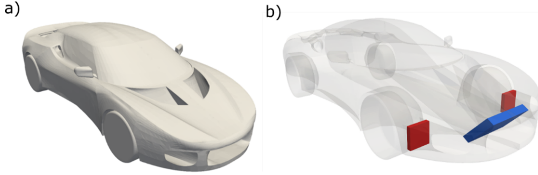
Fig. 10. 'Base' case model: a) Plain geometry b) Transparent view showing the HEs.
