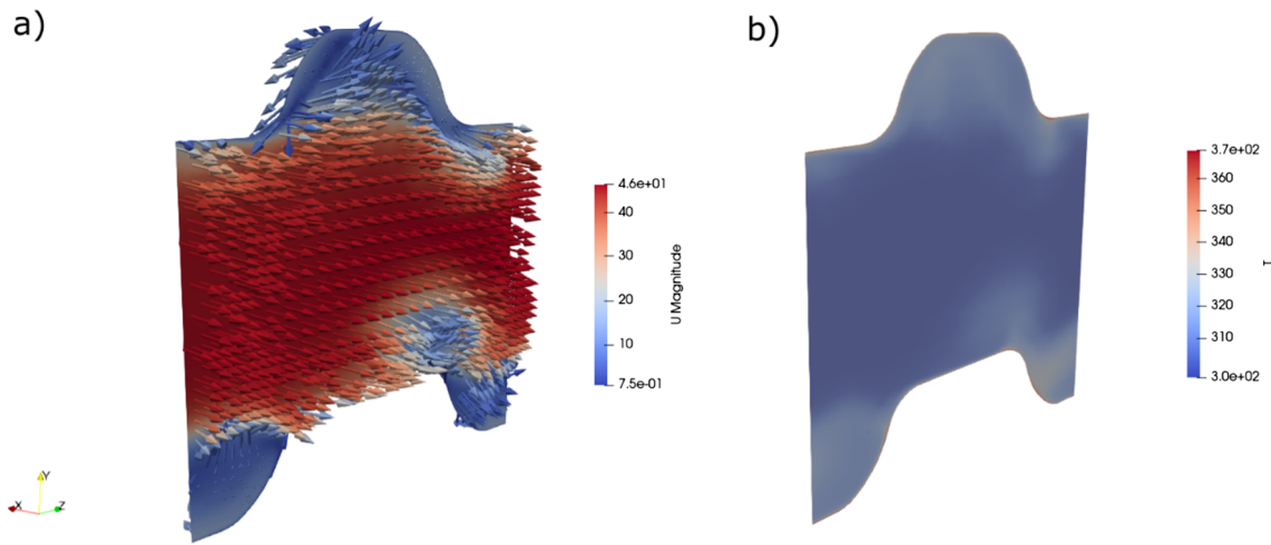
Fig. 8. Cross-sectional view a) Velocity field [m/s], b) Temperature field [K].
