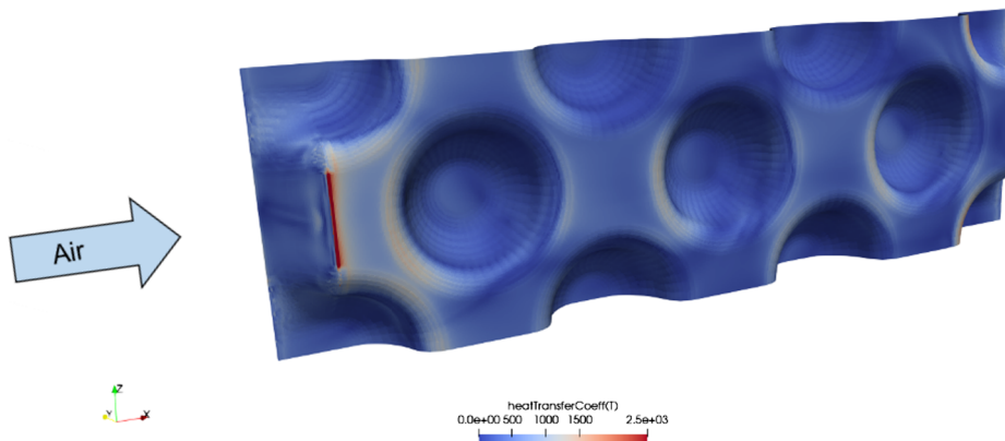
Fig. 9. Heat Transfer Coefficient ( h_c ) contours on the HE shell.
