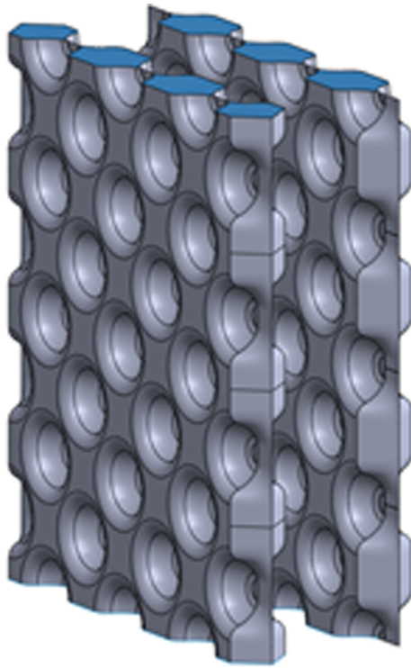
Fig. 1. Heat Exchanger portion.
