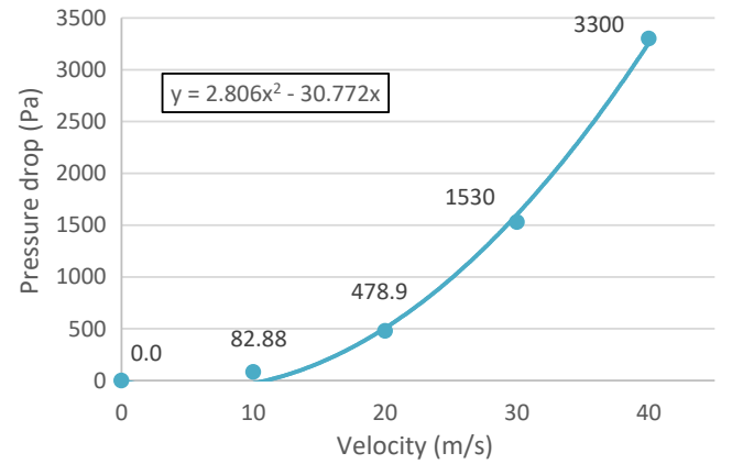
Fig. 4. Pressure drop chart.
