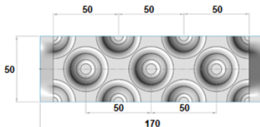
Fig. 2. HE's characteristic dimensions (mm).
