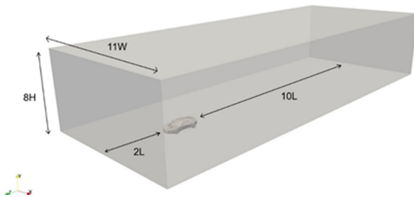
Fig. 13. Computational domain.
