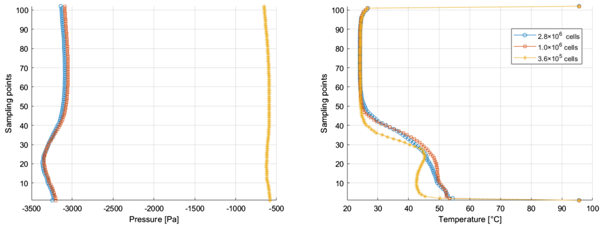
Fig. 7. Mesh independence study on pressure and temperature.
