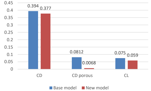
Fig. 16. Comparison between the different aerodynamic coefficients of drag, drag porous, and lift for the 'base' and 'new' models.
