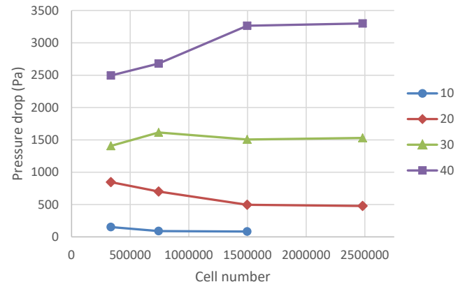
Fig. 3. Mesh independence study for the HE dynamic analysis.
