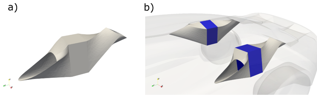
Fig. 12. Rear ducts: a) Single duct view b) Rear positioning of the HEs.
