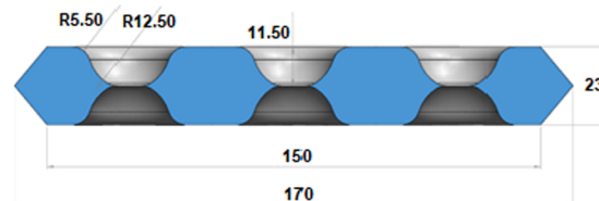
Fig. 2. HE's characteristic dimensions (mm).
