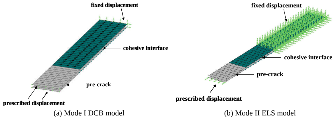
Figure 3: Delamination models.
