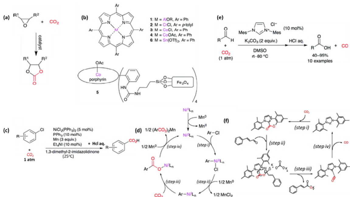
Fig. 13. (a) The combination of CCs by epoxides and CO 2 . (b) Metalloporphyrin catalysts 1-6. Reprinted with permission from Ref. [204]. (c) Nickel-catalyzed carboxylation and (d) reasonable reaction pathways. Reprinted with permission from Ref. [211]. (e) The NHC-catalyzed and (f) reaction mechanism reduction of CO 2 . Reprinted with permission from Ref. [212].
