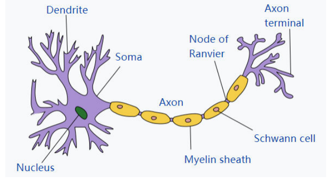
Fig. 1. The basic composition of a neuron [22].
