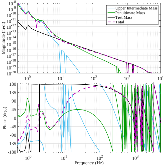
FIG. 4. Overall actuation transfer function A(f) and actuation functions for each suspension stage F_i(f) \mathcal{K}_i A_i(f) for the L1 detector. The mechanical response of the pendulums and F_i dictate the characteristics of each stage. The strongest actuator, that for the upper intermediate mass, is used below a few Hz. Above \sim 30 Hz, only the test mass actuator is used. At certain frequencies (e.g., 10, 14, and 500 Hz), digital notch filters are implemented for high quality factor features of the pendulum responses in order to avoid mechanical instabilities. The H1 actuation function differs slightly in scale, frequency dependence, and digital filter choice.
