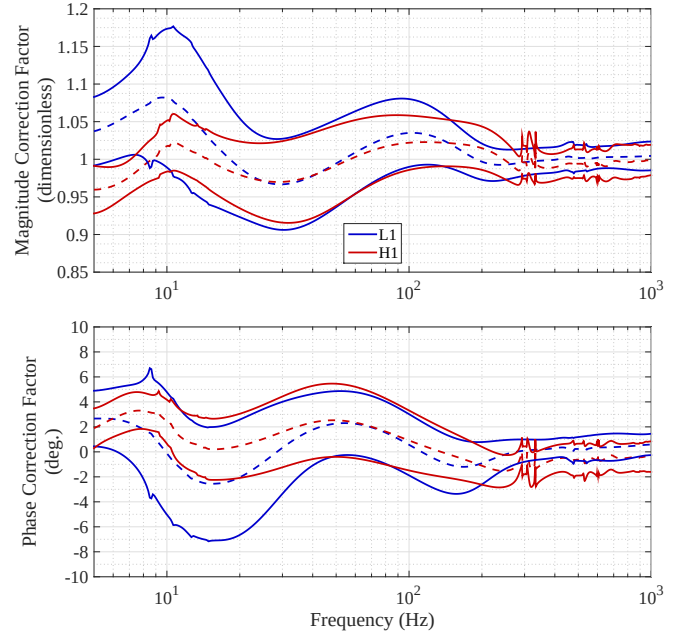
FIG. 8. Known systematic error and uncertainty for the response function R(f) at the time of GW150914, expressed as a complex correction factor 1 + \delta R(f, t)/R(f) (dashed lines) with surrounding uncertainty \pm \sigma_R(f) (solid lines). The upper panel shows the magnitude, and the lower panel shows the phase. The solid lines define the 68% confidence interval of the precision and accuracy of our estimate of h(t) .
