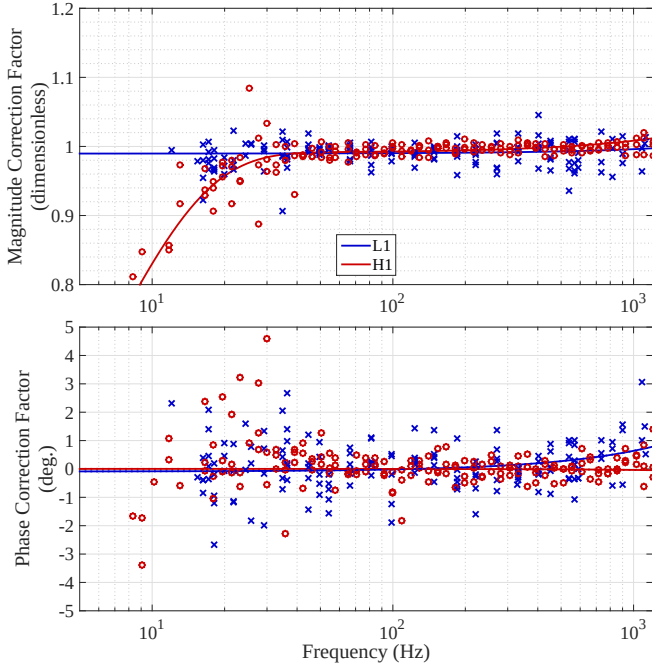
FIG. 7. Measured frequency-dependent sensing function correction factors, \zeta_i^{(\text{fd})} , for L1 (blue crosses) and H1 (red circles) and their fits, \zeta_i^{(\text{fd,fit})} .
