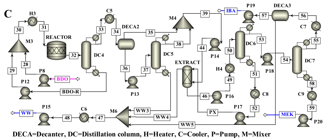
Fig. 4. Process flowsheet for the conversion of 2,3-butanediol (BDO) to methyl ethyl ketone (MEK). Separation of MEK-water using (A) heterogeneous azeotropic distillation (Configuration I), (B) extraction-distillation (Configuration II), and (C) separation of MEK-IBA-water using extraction-distillation (Configuration III).
