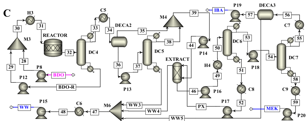
Fig. 4. Process flowsheet for the conversion of 2,3-butanediol (BDO) to methyl ethyl ketone (MEK). Separation of MEK-water using (A) heterogeneous azeotropic distillation (Configuration I), (B) extraction-distillation (Configuration II), and (C) separation of MEK-IBA-water using extraction-distillation (Configuration III).
