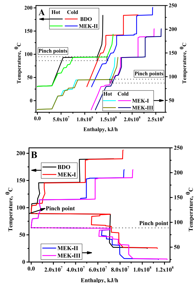
Fig. 5. (A) Composite and (B) grand composite diagram.
