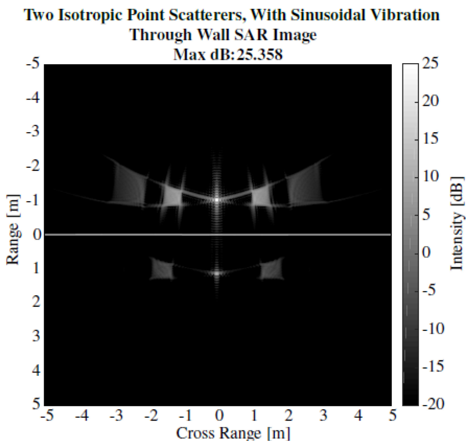
Figure 3: Monostatic SAR simulation of two vibrating isotropic point scatterers located before and after a single concrete medium, highlighted by the white rectangle (this is not part of the SAR image).
