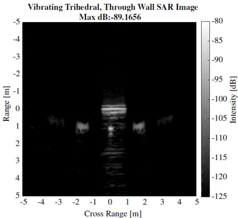
Figure 7: Measurement SAR image of a trihedral located behind the breezeblock wall (as shown in Figure 5) following a sinusoidal motion.
