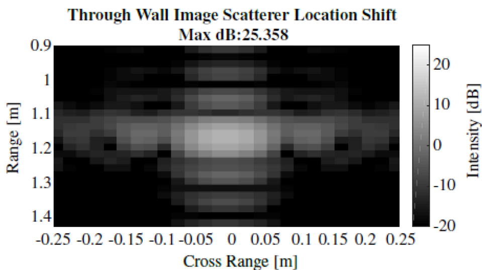
Figure 4: Zoomed in region of Figure 3, highlighting the artificial location shift down range, for the scatterer located behind the wall. This can be seen to be \approx 0.15 [m], from its actual location of [0, 1] [m].
