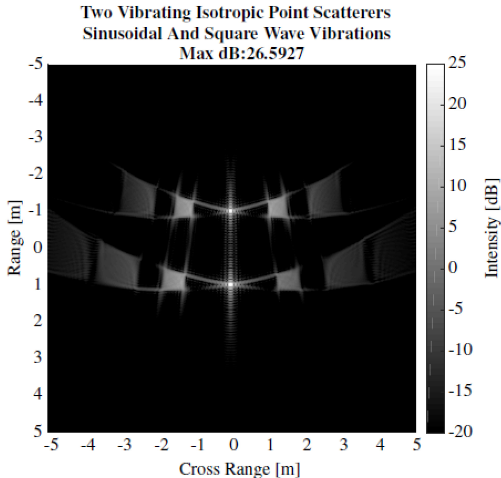
Figure 2: SAR image of two vibrating isotropic points scatterers in a vacuum. One scatterer is located at [0, 1] [m] and has a square wave vibration and the second is located at [0, -1] [m] and has a sinusoidal vibration.
