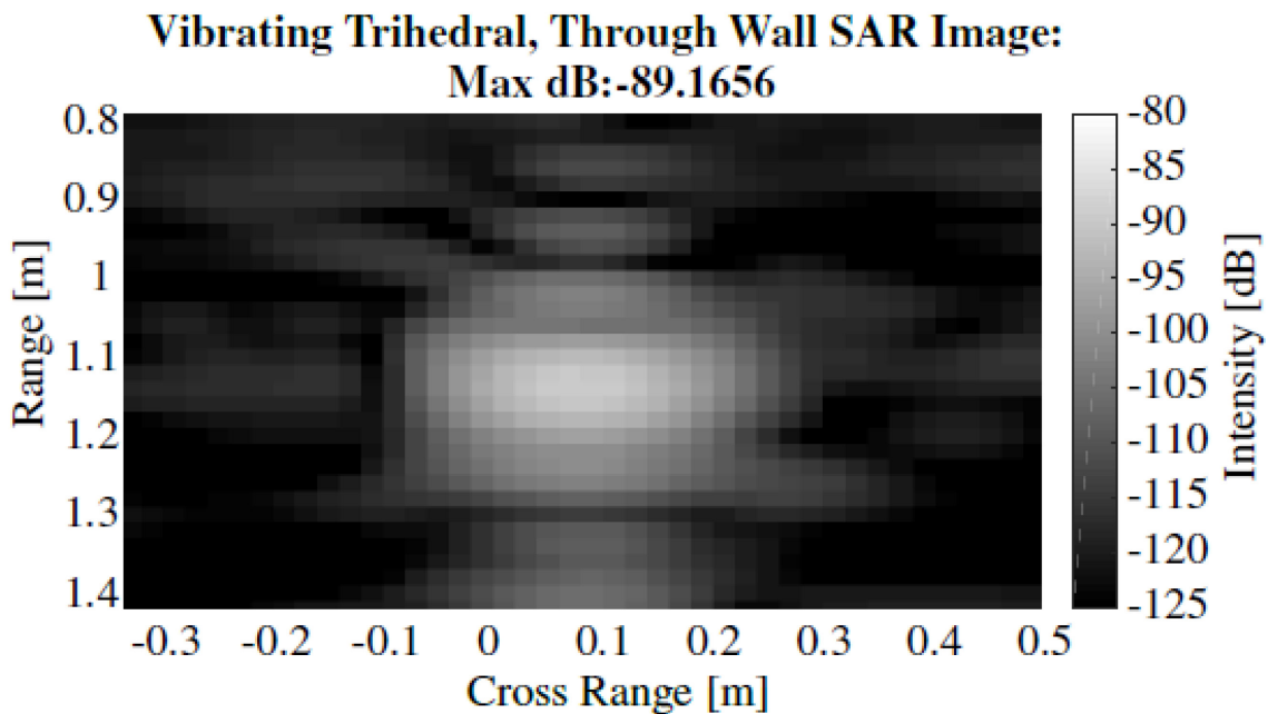
Figure 8: Zoomed in region of Figure 7, highlighting the artificial location shift down range. This can be seen to be \approx 0.18 [m], from its actual location of [0, 1] [m].
