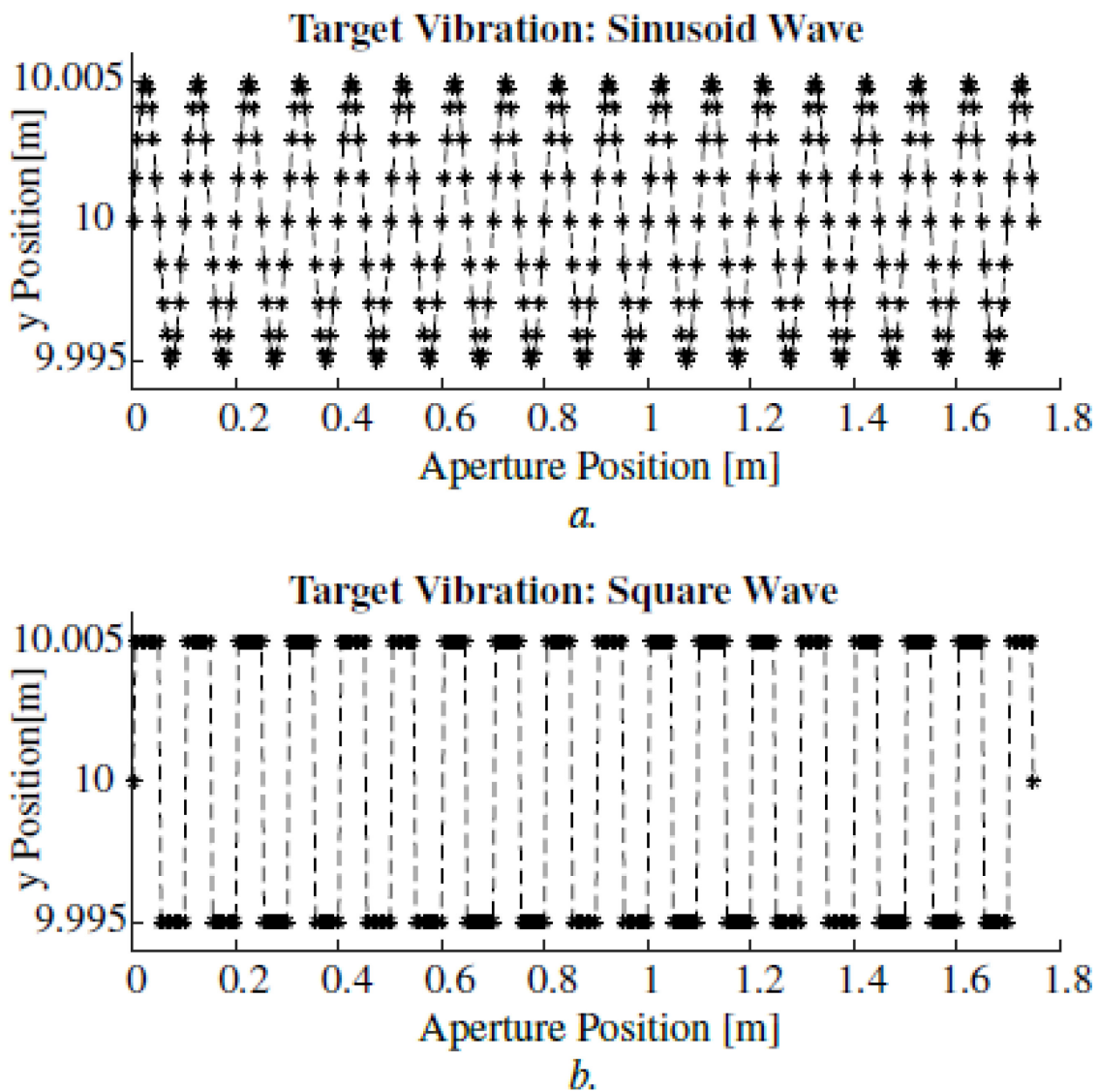
Figure 1: Example vibrational outputs from equations (2) and (3): (a) Sinusoid vibration; (b) Square wave vibration.
