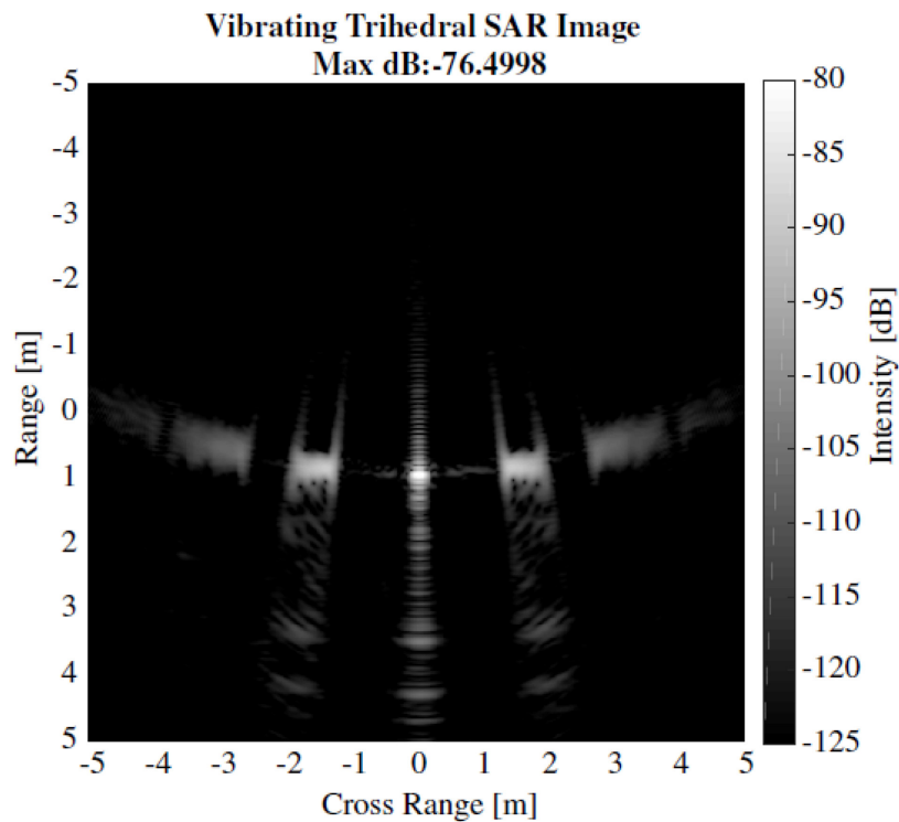
Figure 6: SAR image of a trihedral target following a sinusoidal motion, measured without obstruction. The vibration has a 5 [mm] amplitude and 10 [Hz] frequency, therefore emulating a 1.7 [sec] flight time, if the antennas were moving with a constant velocity across the 3.5 [m] aperture.
