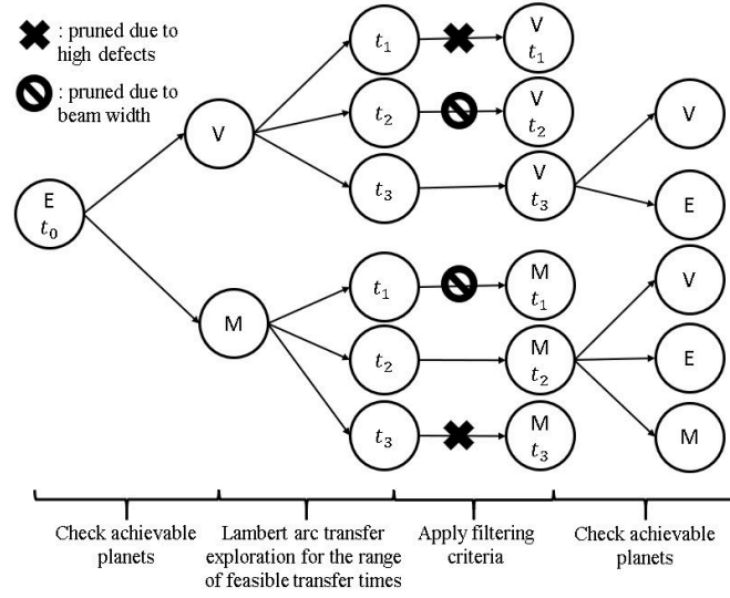
Figure 3: Tree expansion for automatic MGA solution as done by ASTRA's Process 1. 'E', 'V' and 'M' stand for Earth, Venus and Mars, respectively, while t_i with i = 0, 1, \dots refers to epoch at which the planet is visited. Reference to planets and dates are given for example purposes only.
