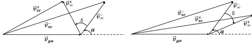
Figure 2: Heliocentric velocity change due to swing-by in front of the planet (left image), and behind the planet (right image). Left and right cases result in minimizing and maximizing the energy after the swing-by, respectively. The angle \alpha is a geometry parameter used to describe minimum/maximum energy post swing-by.
