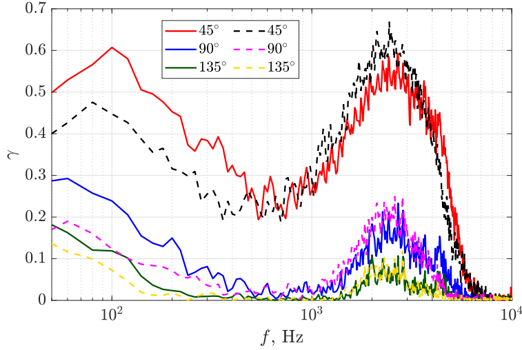
Fig. 8 Coherence results measured at x/D_j = 2 , r/D_j = 1.1 . Solid lines for round jet, dashed lines for zigzag jet results
