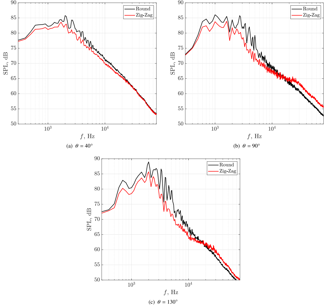
Fig. 4 Installed jet sample SPL spectra. Nozzle with lip treatment (red) and untreated baseline (black) are shown. Jet acoustic Mach number is equal to 0.6
