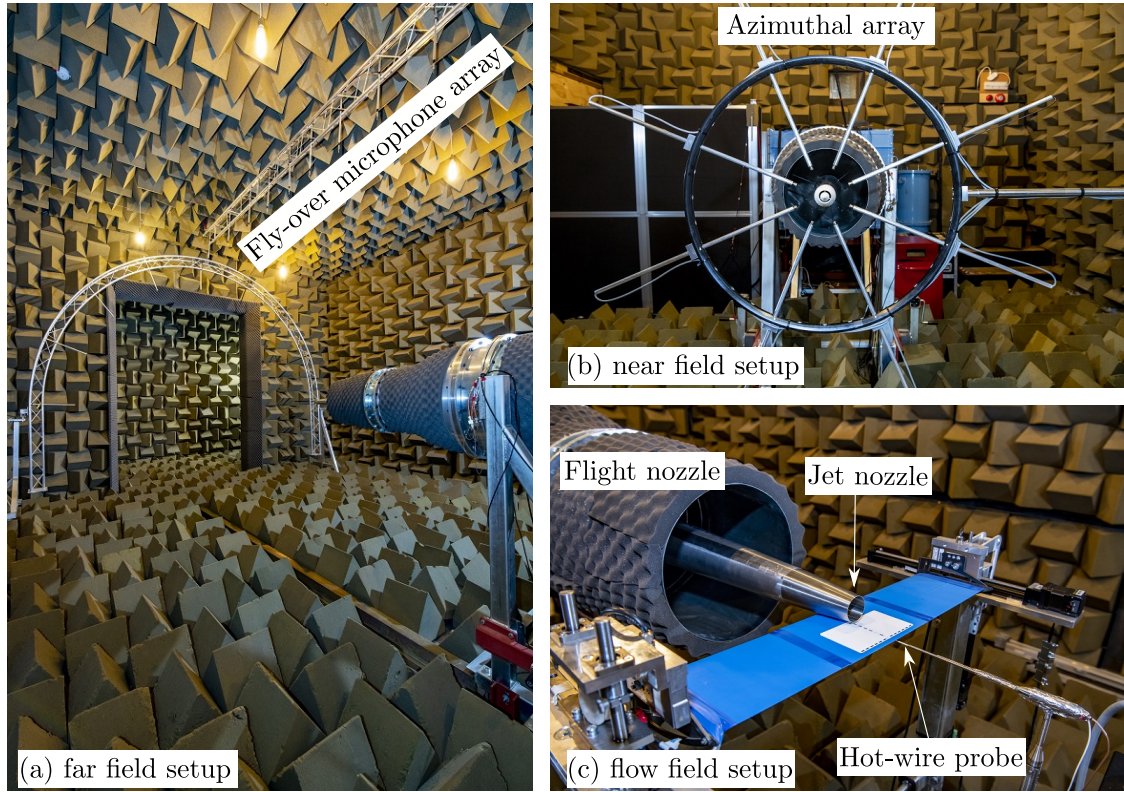
Fig. 1 The Flight Jet Rig in the Doak Laboratory, at the University of Southampton
