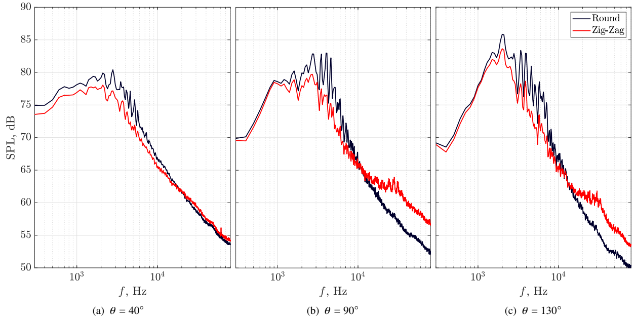
Fig. 5 Installed jet in-flight SPL results. Jet acoustic Mach number is equal to 0.6, flight-stream Mach number 0.1
