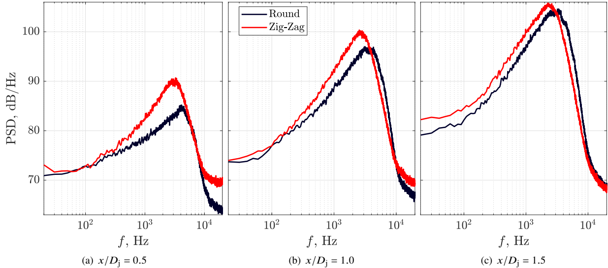
Fig. 6 Near-field PSD data at three axial locations. M_j = 0.6 , r/D_j = 0.8
