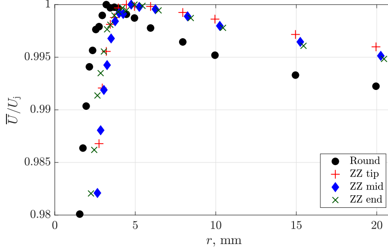
Fig. 10 Mean velocity profiles measured close to the exit plane (focused on the vena contract region)
