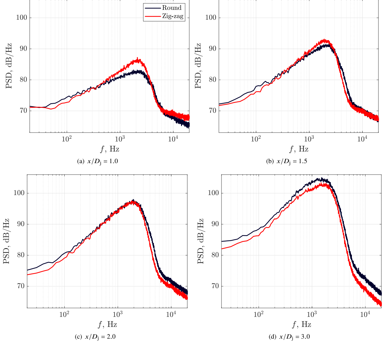
Fig. 7 Near-field PSD data at four axial locations. M_j = 0.6 , r/D_j = 1.1
