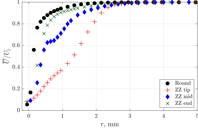
Fig. 9 Mean velocity profiles measured close to the exit plane of the baseline and zigzag nozzles
