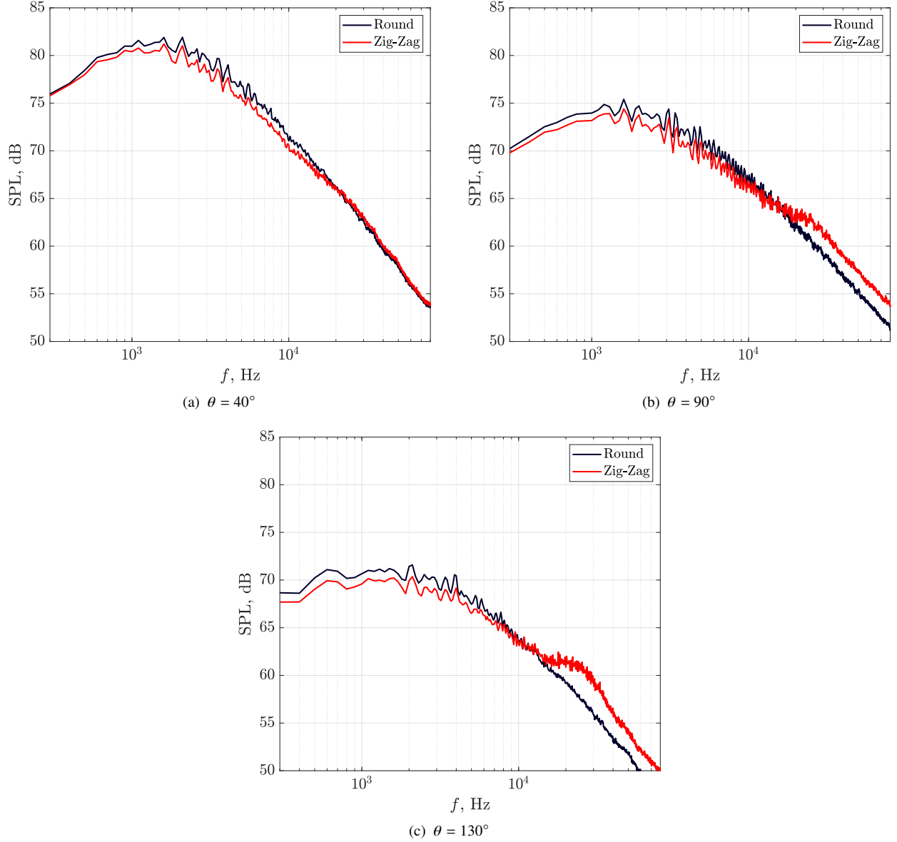
Fig. 3 Isolated jet configuration sample SPL results. Nozzle with lip treatment (red) and untreated baseline (black) are shown. Jet acoustic Mach number is equal to 0.6
