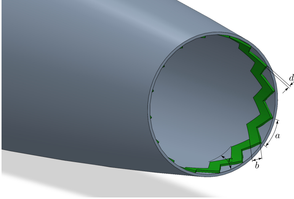
Fig. 2 Schematic showing the zigzag lip treatment used in this work
