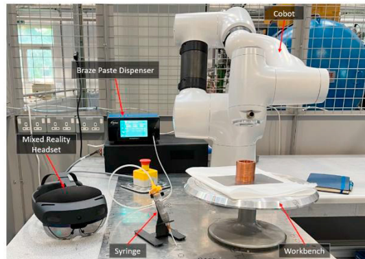
Fig. 4. Use case brazing cell at TWI Ltd
