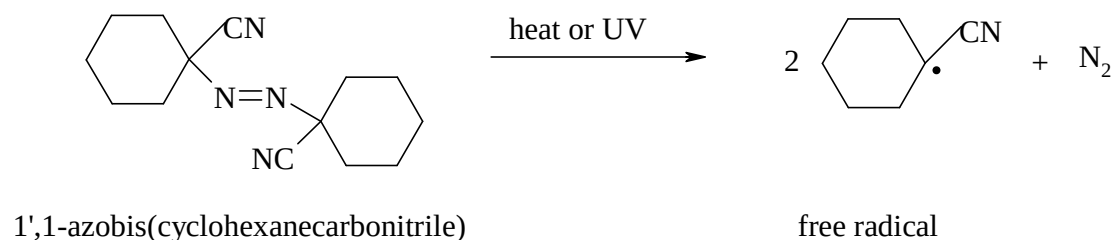
Figure 1. Mechanism of decomposition for 1',1-azobis(cyclohexanecarbonitrile), based on the mechanism of decomposition of AIBN. 12
