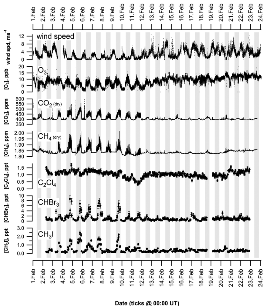
FIG. 6. Surface observations of (top to bottom) wind, O_3 , CO_2 , CH_4 , C_2Cl_4 , CHBr_3 , and CH_3I at the ARM facility on Manus from 1 to 24 Feb 2014. The time shown along the x axis is universal time. The shading indicates the local time, with the darker bands representing nighttime.
