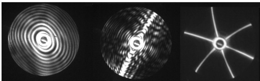
FIG. 8. AIITS scattering patterns recorded from ice particles in the upper troposphere–lower stratosphere (UTLS), at altitudes of about 16 km and temperatures of about -80^{\circ}\text{C} . The pictures are indicative of (left) a smooth quasi-spherical ice particle, (center) a columnar crystal, and (right) a pristine hexagonal plate.
