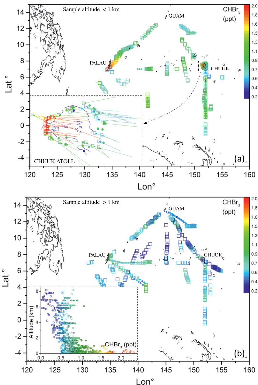
FIG. 5. CHBr 3 mixing ratios (colors) sampled by the FAAM aircraft during CAST using the whole air sampler (squares) and the onboard GC-MS (circles). (a) All measurements made at altitudes less than 1 km. The enlarged inset shows the values around the Chuuk atoll. The lines associated with each measurement in the inset indicate the instantaneous wind speed measured by the aircraft. (b) The measurements at altitudes greater than 1 km. The inset shows the vertical profile of all measurements.
