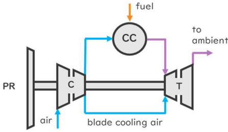
Figure 1: Baseline mGT plant layout.
