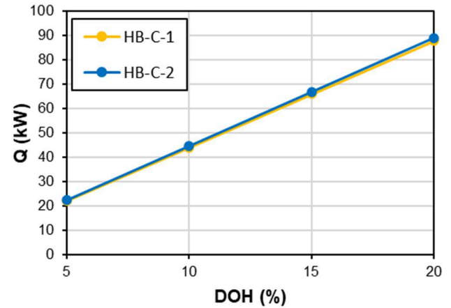
Figure 9: Relationship between heat exchanged by the HEX ( Q ) and degree of hybridization (DOH) for cruise (for this case study).
