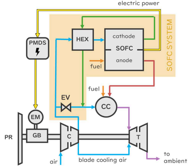
Figure 3: HB-2 plant layout (mGT-SOFC system with expansion valve).
