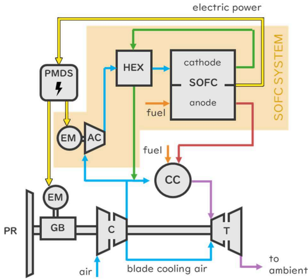
Figure 2: HB-1 plant layout (mGT-SOFC system with auxiliary compressor).
