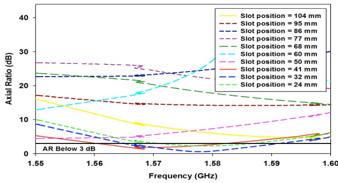
Fig 7. Simulated axial ratio of slot positioning.
