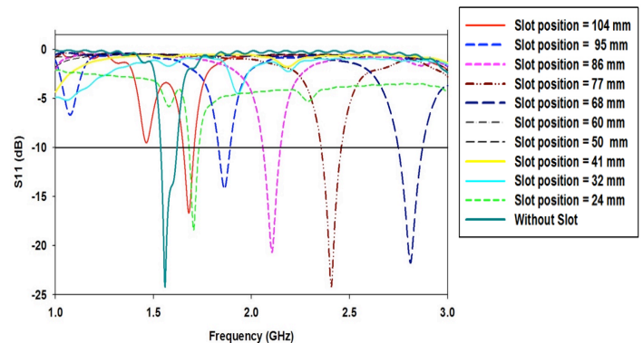
Fig 6. Simulated reflection coefficient with different slot positions.
