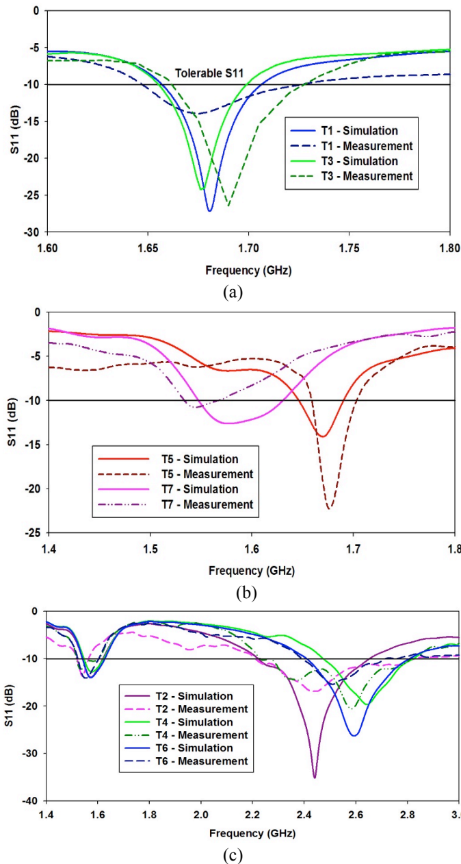
Fig 10. Simulated and measured reflection coefficients for different configurations: a) T1 and T3, b) T5 and T7 and c) T2, T4 and T6.
