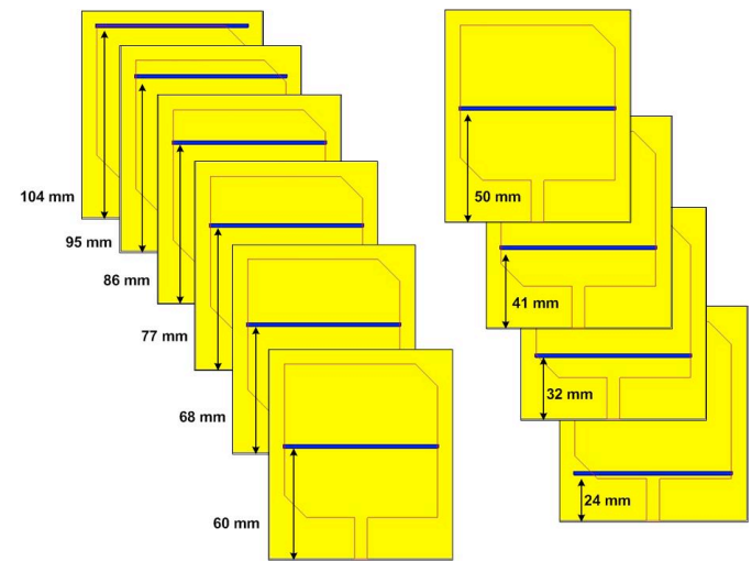
Fig 5. Analysis of slot positions on the ground plane.
