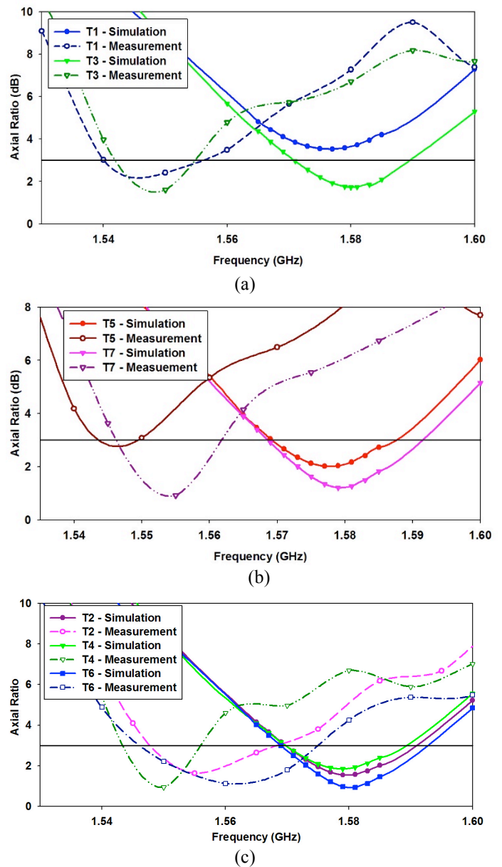
Fig 11. Simulated and measured axial ratios for different configurations: a) T1 and T3, b) T5 and T7 and c) T2, T4 and T6.
