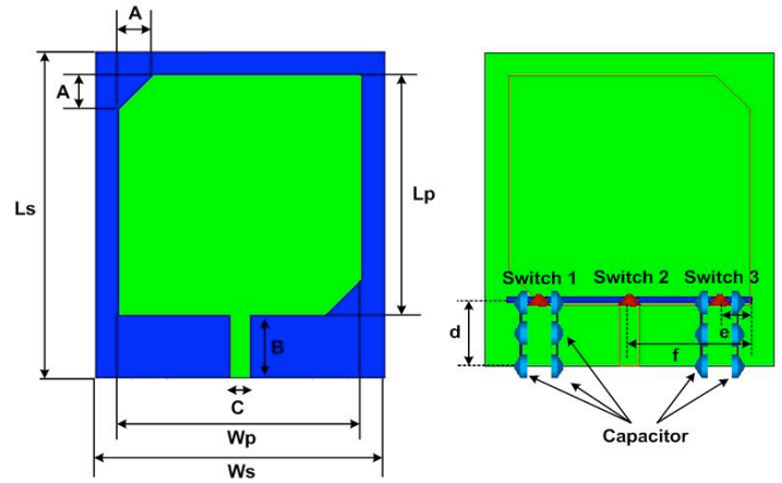
(a) Front view (b) Back view Fig 8. Geometry of the proposed antenna. (a) front view and (b) back view.
