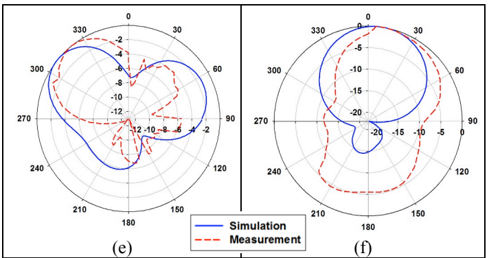
Fig 13. Simulated and measured radiation pattern. (a) T2 at 1.57 GHz, xy-plane cut, (b) T2 at 1.57 GHz, yz-plane cut, (c) T2 at 2.45 GHz, xy-plane cut, (d) T2 at 2.45 GHz, yz-plane cut, (e) T7 at 1.57 GHz, xy-plane cut, and (f) T2 at 1.57 GHz, yz-plane cut.
