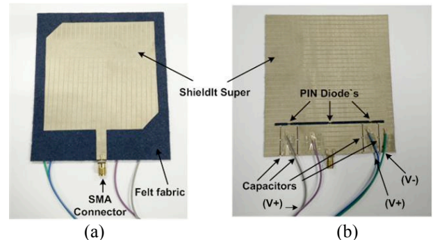
(a) (b) Fig 9. Photograph of the fabricated antenna. (a) front view. (b) back view.
