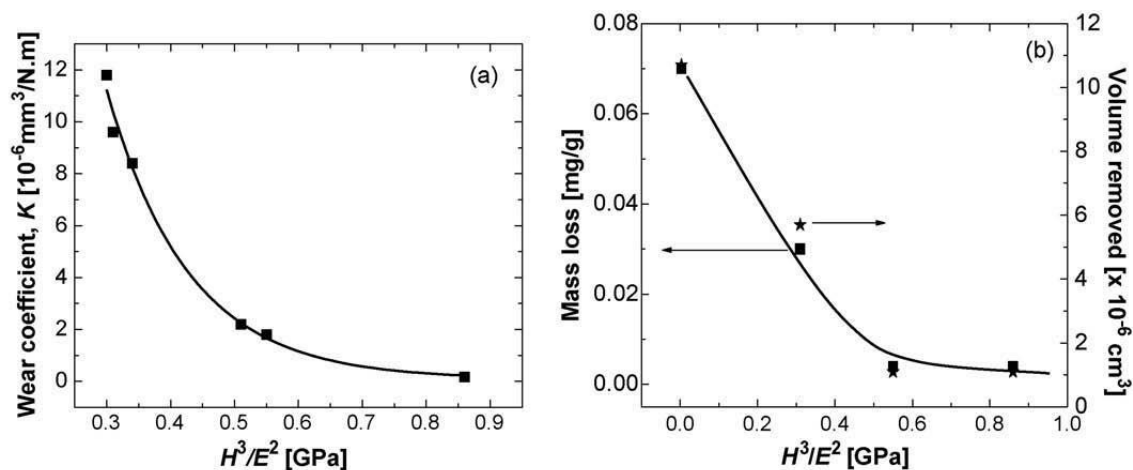
Figure 11. Tribological characteristics of TiN and nanocomposite nc-TiN/SiN 1.3 films as a function of the H^3/E^2 ratio: (a) wear coefficient; (b) erosion rate [135].
