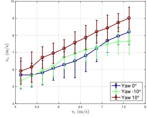
Fig. 4. The average nacelle anemometer wind speed ( v_n ) per meteorological tower cup anemometer wind speed ( v_c ) intervals of 0.25 m/s. Bins with more than 50 measurements are kept.
