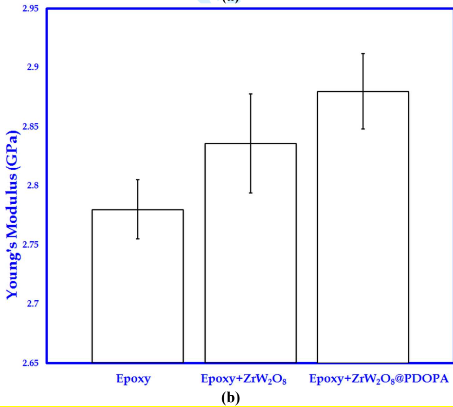
Figure 8 (a, b) Comparative tensile strength and Young's modulus results of the pristine epoxy and ZrW 2 O 8 / ZrW 2 O 8 @PDOPA) nanocomposites.
