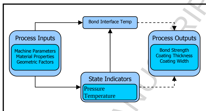
Fig.1. Diagrammatic representation of process parameters
