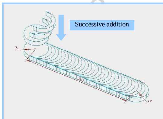
Fig.7. Composite geometric model of deposit layer and substrate
