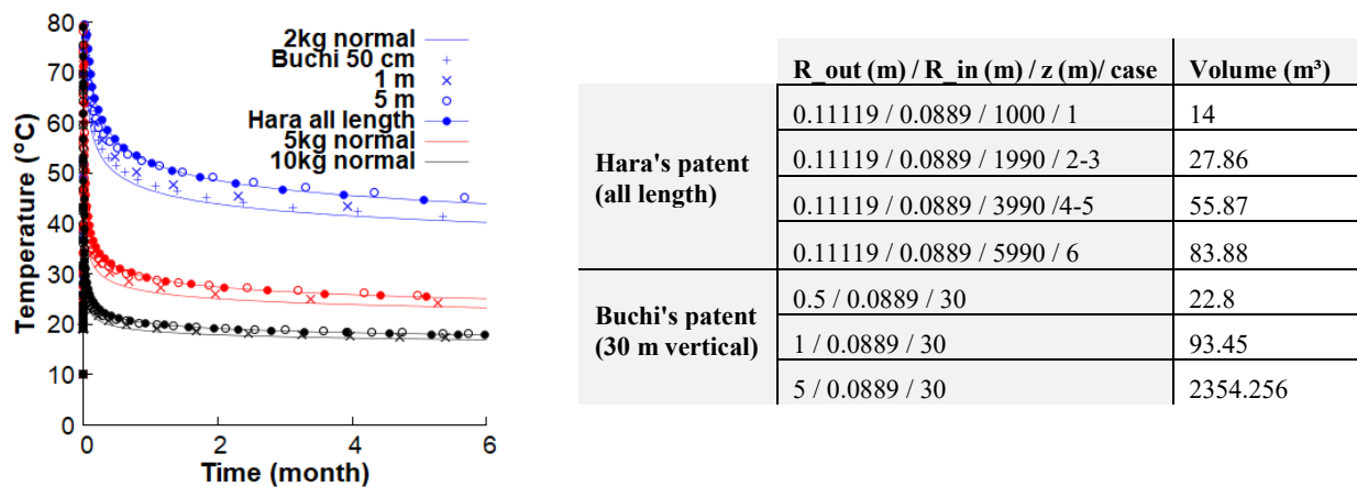
Figure 7: (Left) Produced water temperature during 6 months for the case 1 with different mass flow injection following the radial length of graphite along the wellbore ( r ) and z = 30 . The simulated results are higher than 100^\circ\text{C} but the vertical axis has been limited to 80^\circ\text{C} to observe the long-term temperature difference between the cases. (Right) Volume of Graphite needed for different diameters and length in the Hara and Buchi's patent.
