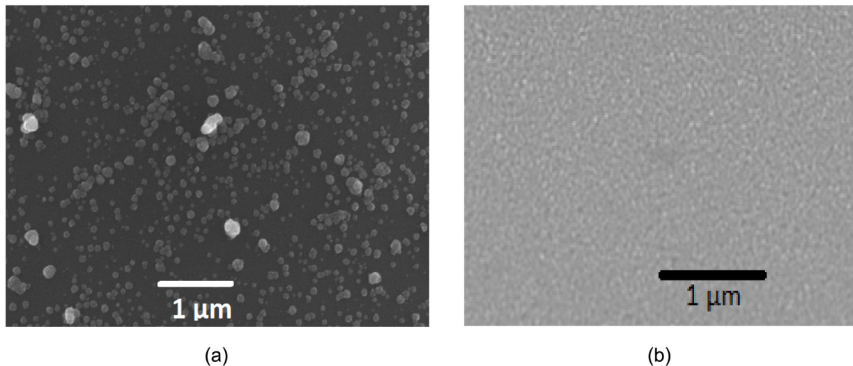
Fig. 2. SEM images of coatings of (a) TiO 2 and (b) TMPyP-TiO 2 deposited onto glass microscope slides with the liquid phase deposition approach outlined in Section 3.1. In both cases, the glass slide had been kept in the film-forming solution for five hours.
