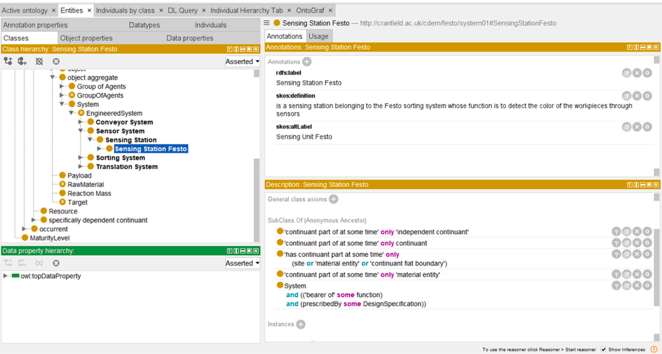
Fig. 11. Screenshot of the Protégé tool focusing on the class Sensing Station Festo.
