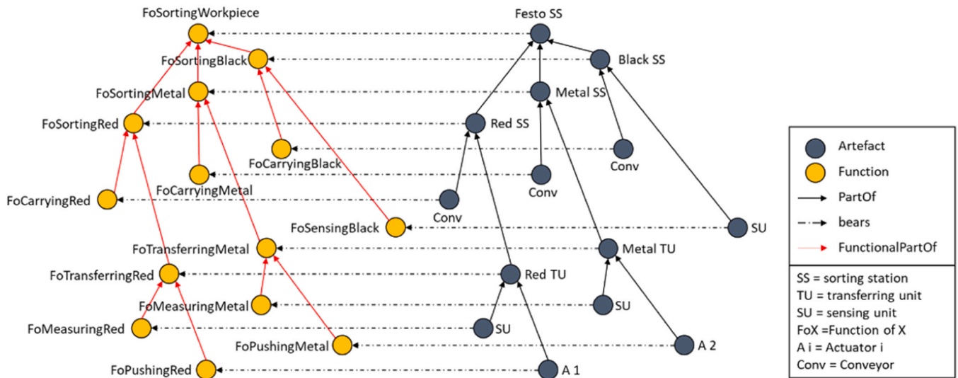
Fig. 8. Mereotopological representation of the system along with functions.
