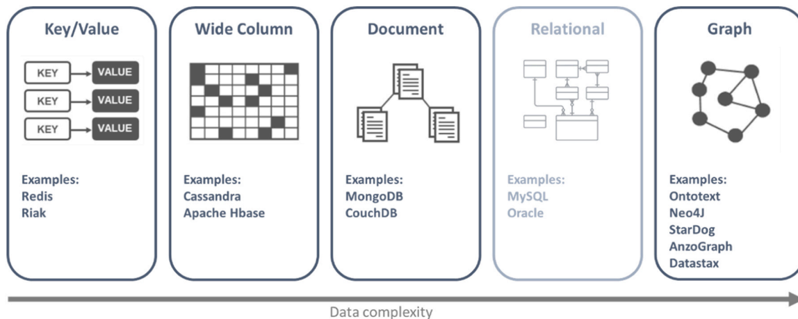
Fig. 5. Database approaches based on data complexity (Inspired from An Introduction to Graph Data Stores and Applicable Use Cases, Sumit Pal, Gartner Research, Published: 24 January 2019, https://www.gartner.com/en/documents/3899263 (accessed 30/06/2023)).
