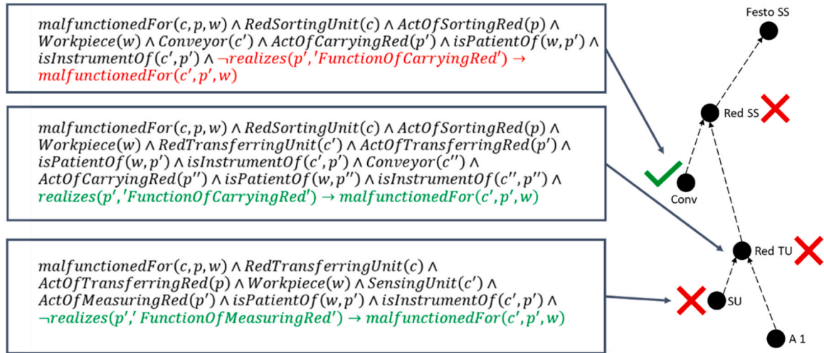
Fig. 21. Visual application of the rules into the system composition.
