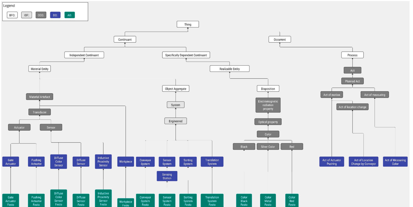
Fig. 10. Overall structure of the ontology.
