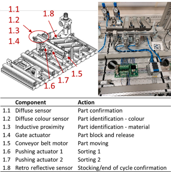
Fig. 7. Festo Sorting Station, schema, components, actions.
