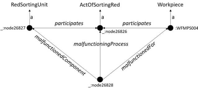
Fig. 18. Schema for the reification.
