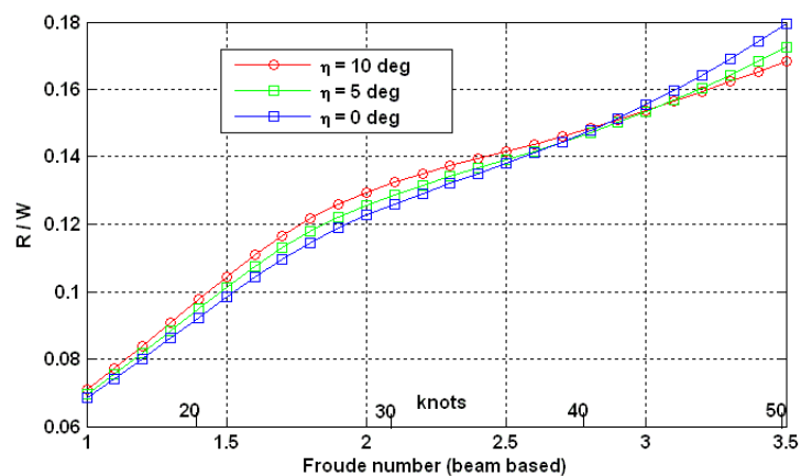
Figure 3: influence of \eta on the resistance to weight ratio
