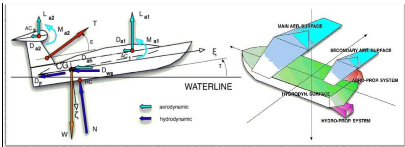
Figure 1: Hybrid Vehicle selected configuration
