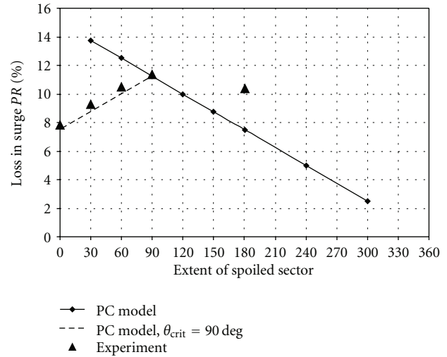
FIGURE 3: Conventional and corrected PC models against experimental data from [8].
