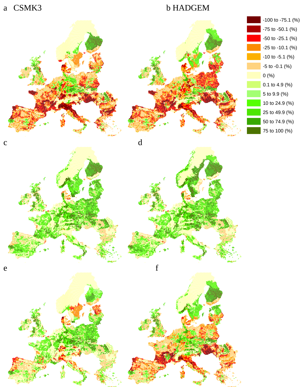
Figure 3 Intensive agricultural land use in 2050 for two climates and two scenarios a) CSMK3+” We are the World” b) HADGEM+” We are the World” c) CSMK3+”Should I Stay or Should I go” d) HADGEM+”Should I Stay or Should I go” e) c with yield +15% f) b with population +25%
