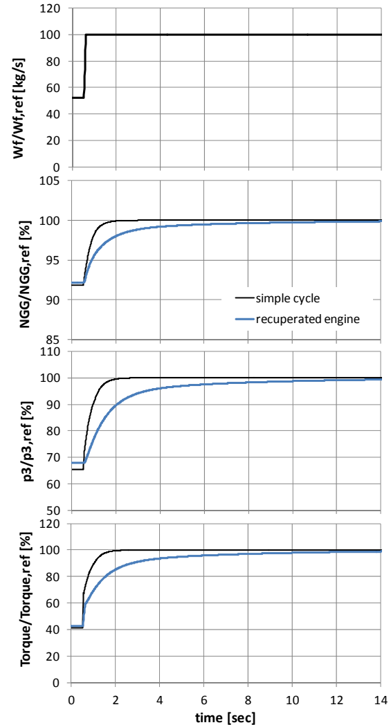
Figure 11: simple cycle and recuperated engine response to a fuel step increase
