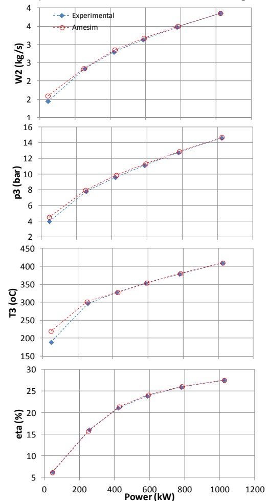
Figure 7: Measured [12] versus calculated data for steady state operation
