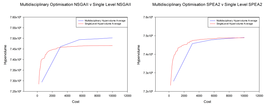
Fig. 13: Bandpass average hypervolume results for the 5 runs of the multidisciplinary optimisation and single level NSGAII and SPEA2 strategies * ( S^U S^M S^L ) [182000, 4150]
