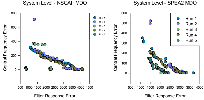
Fig. 11: MEMS bandpass filter run 1 - 5 final population sets for (left) NSGAII multidisciplinary optimisation and (right) SPEA2 multidisciplinary optimisation
