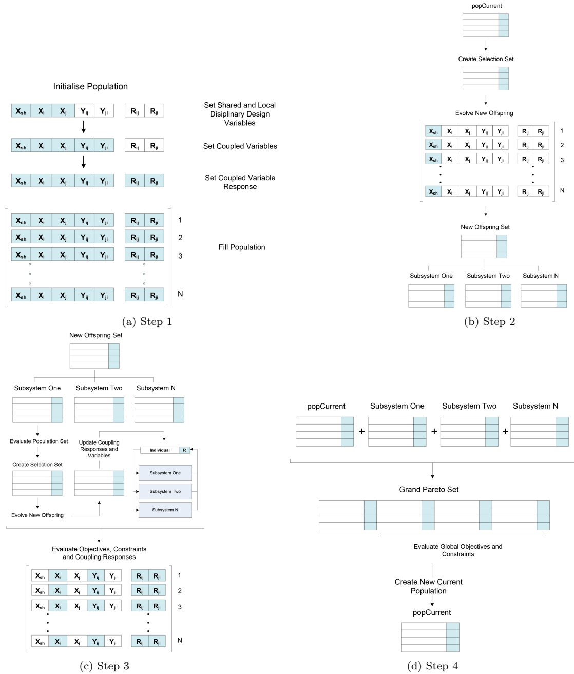
Fig. 5: Multi-objective multidisciplinary optimisation process
