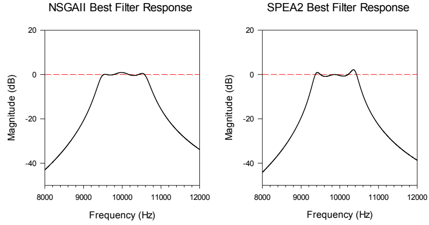
Fig. 12: System level best filter response ranked by filter frequency objective for (left) NSGAII multidisciplinary optimisation and (right) SPEA2 multidisciplinary optimisation
