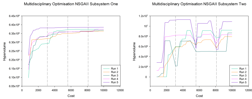
Fig. 15: hypervolume results for the 5 runs of the NSGAII multidisciplinary optimisation strategy for subsystem one (Left) * (S^U \ S^M \ S^L) [4000, 160000] and subsystem two (right) * (S^U \ S^M \ S^L) [12000, 2.0]
