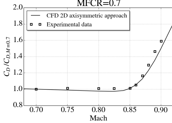
Figure 4: Comparison of nacelle drag as a function of Mach number for the 2D axisymmetric nacelle configuration
