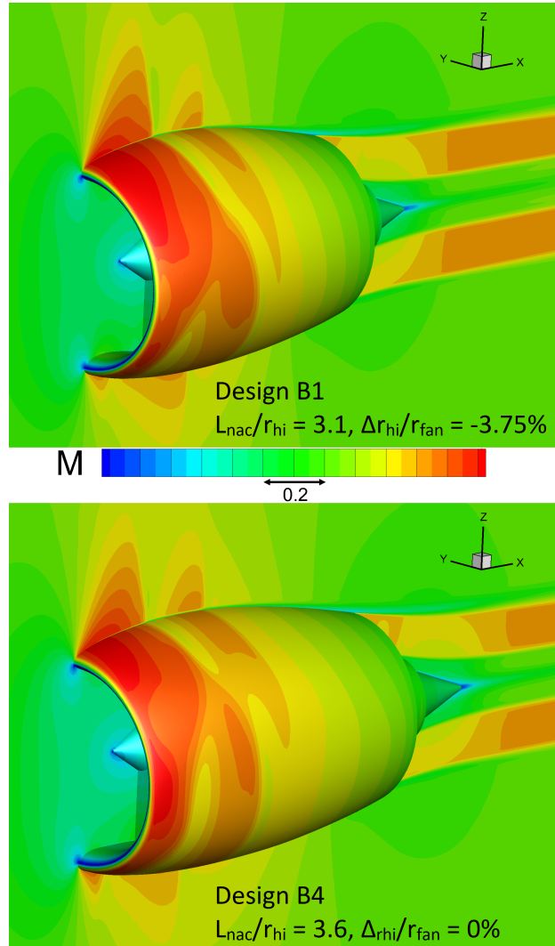
Figure 11: Mach number comparison for the downselected compact design B1 and the baseline architecture B4
