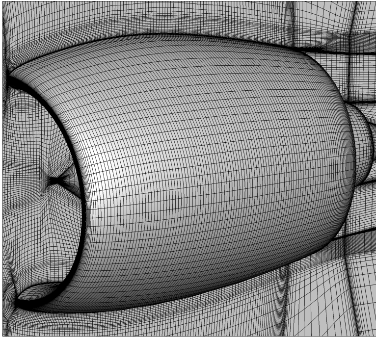
Figure 3: Computational mesh for the 3D numerical model
