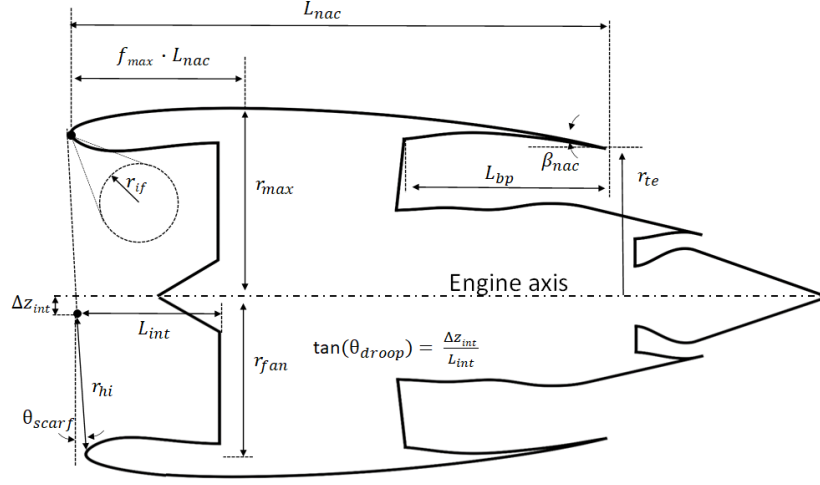
Figure 1: Design variables used to define the aero-engine nacelle
