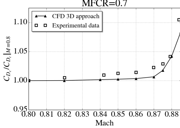
Figure 5: Comparison of nacelle drag as a function of Mach number for the 3D nacelle configuration
