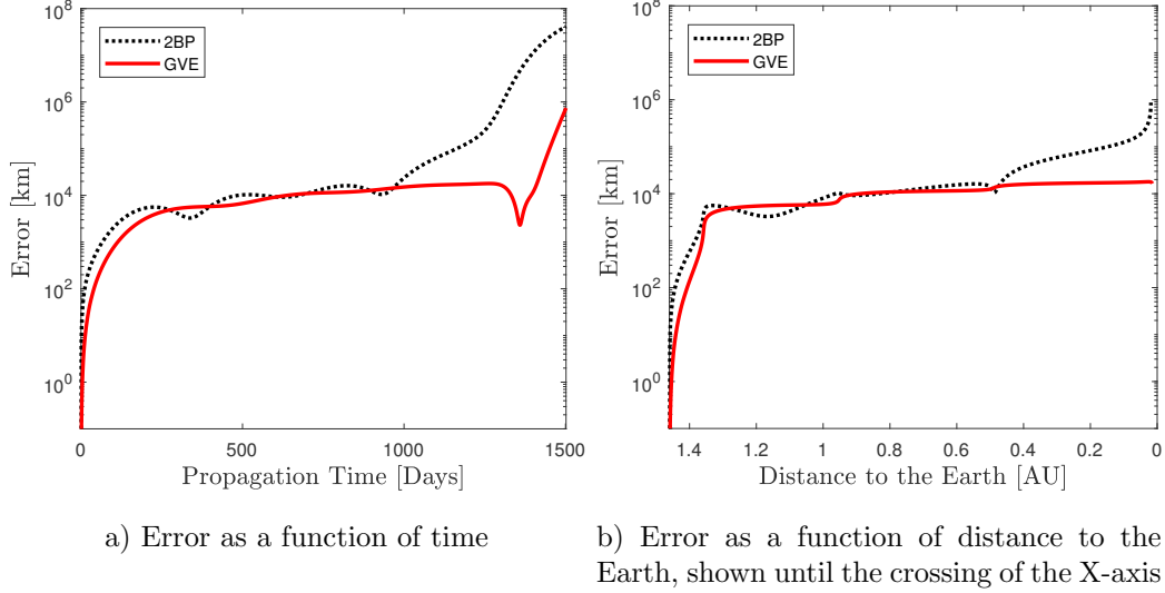
Figure 3: Propagation of the CR3BP, the GVE-3B and 2BP from point A to point B
