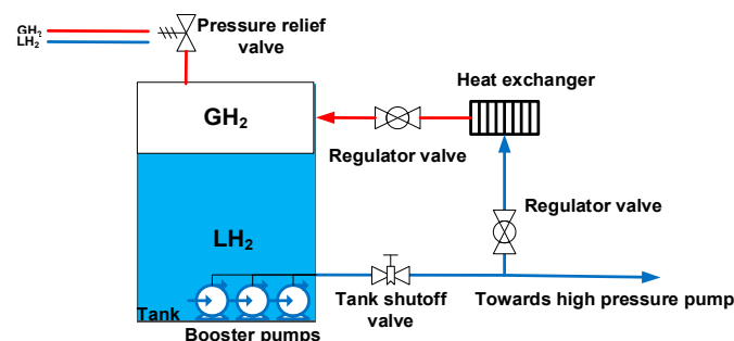
Figure 1. Simple schematic of a low-pressure (airframe) \text{LH}_2 fuel system.
