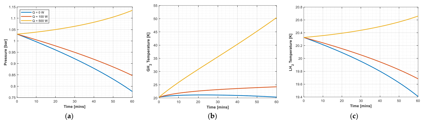
Figure 5. Time evolution for Scenario #2: (a) tank pressure, (b) GH 2 temperature, (c) LH 2 temperature.
