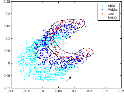
Figure 12: Results from GSVRM for dataset #4.
