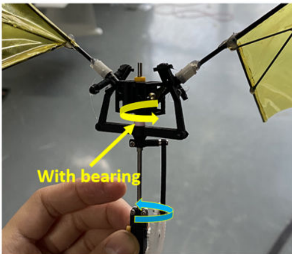
(a)FWR with bearing
