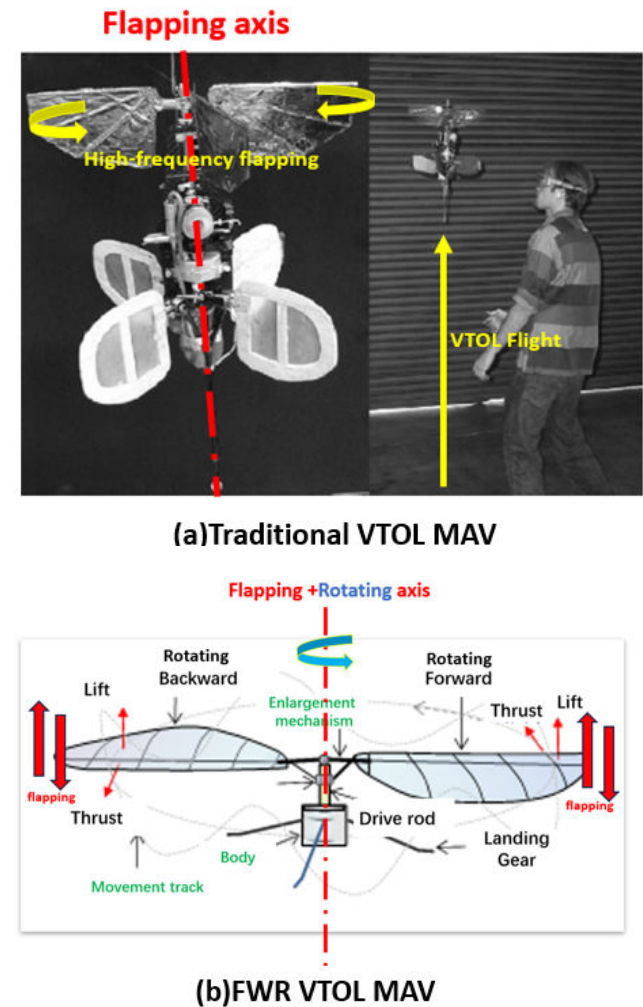
Figure 1 Comparison between Traditional MAV and FWR MAV
