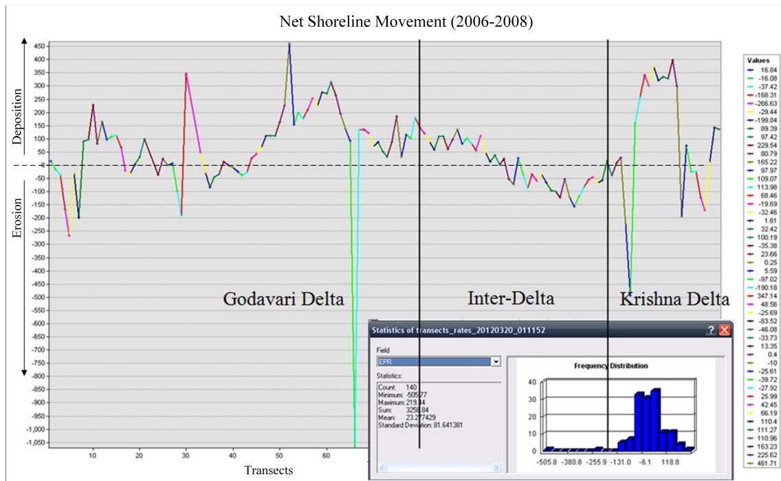
Fig 7 NSM/EPR Trend of Study Area in the period 2006–2008
