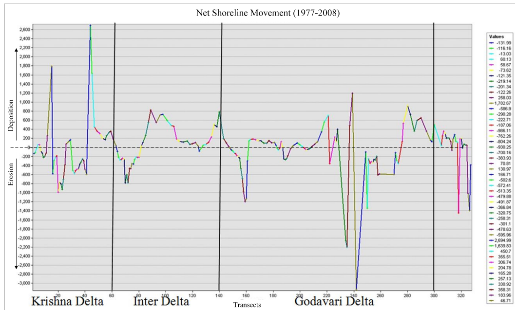
Fig 8 NSM/EPR Trend for K-G Delta (1977–2008)
