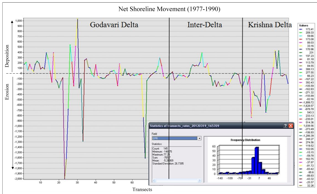
Fig 3 NSM/EPR Trend of Study Area in the period 1977-1990
