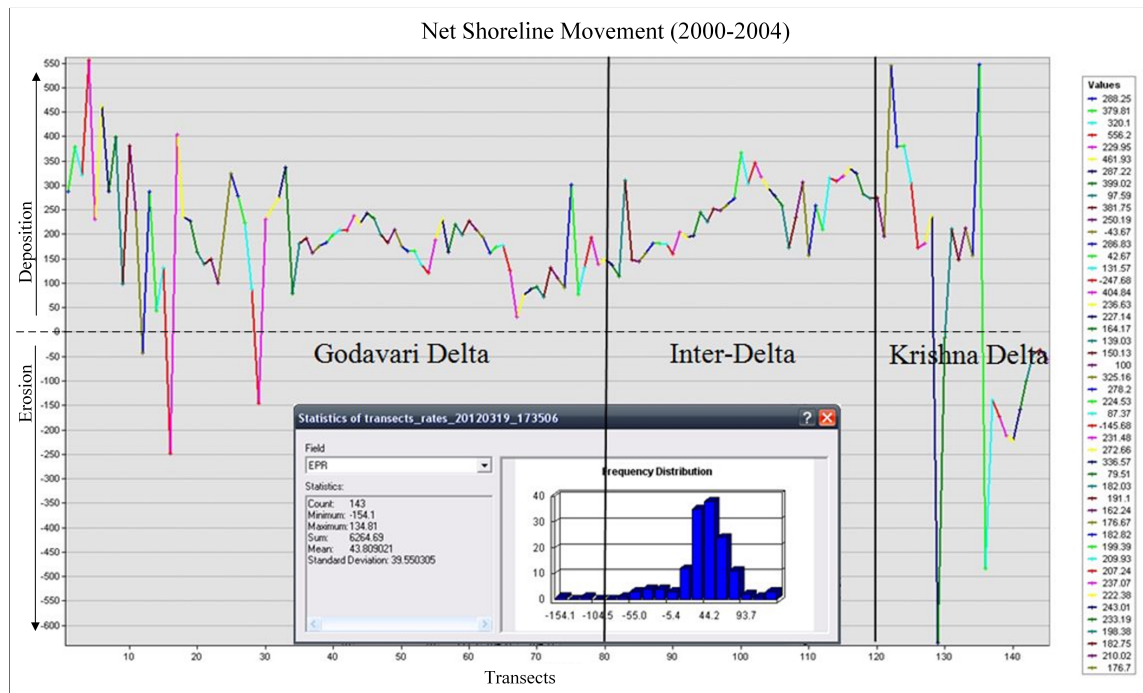
Fig 5 NSM/EPR Trend of Study Area in the period 2000–2004
