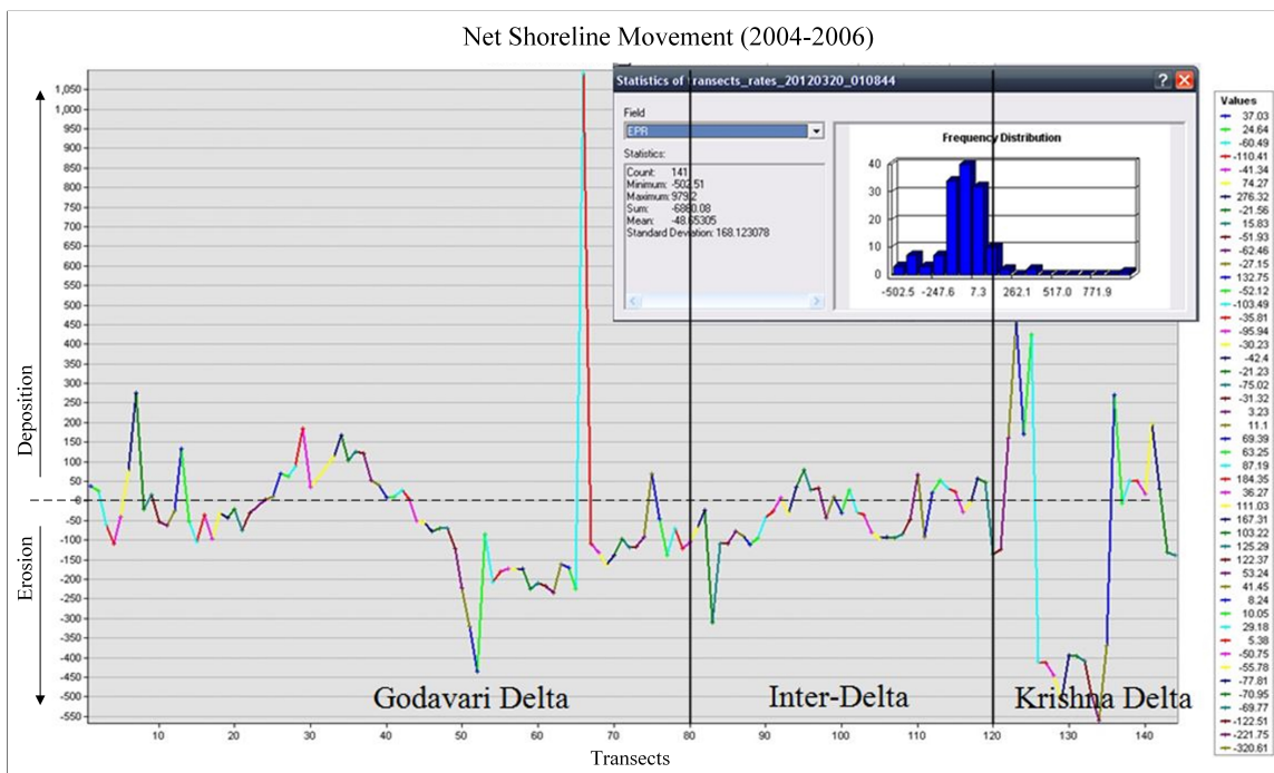
Fig 6 NSM/EPR Trend of Study Area in the period 2004–2006
