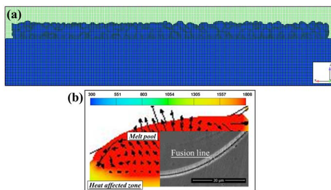
Figure 1. (a) Mesh discretization and (b) Validation of the proposed model. The experiment observation of the melt pool in sub-figure (b) reprinted from [8], Copyright (2021), with permission from Elsevier. (The reader is referred to the web version of this article for a better understanding).
