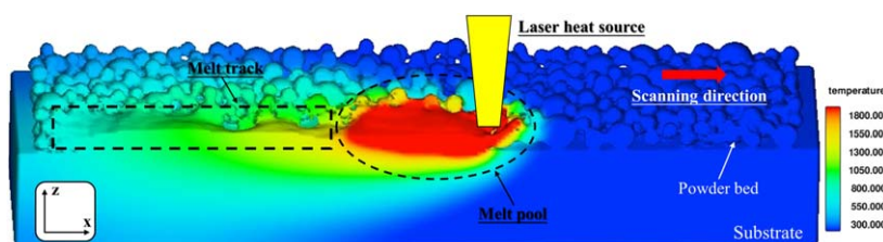
Figure 2. Temperature field, melt pool profile, and melt track morphology at the stable stage in Sul-1, corresponding to the physical time of 1100 \mu\text{s} . The temperature in Kelvin (K) is expressed by the color bar. (The reader is referred to the web version of this article for a better understanding).
