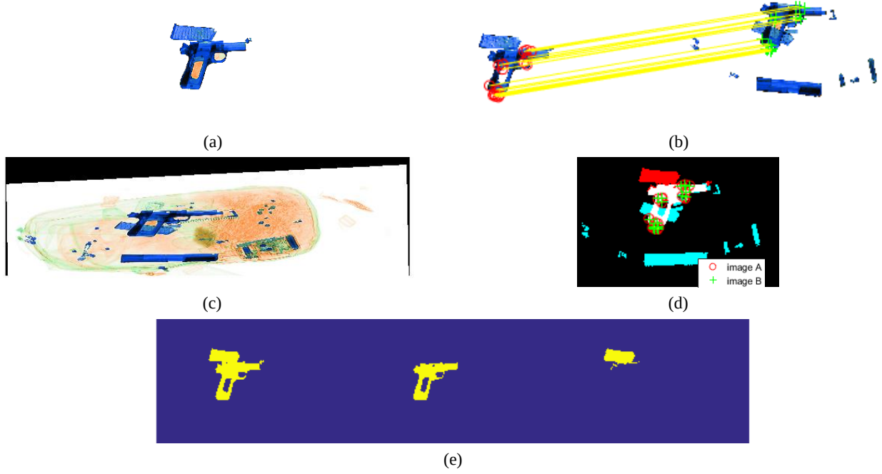
Figure 6. Hard object clustering pipeline (a) cluster Cl_i of image f_{high}^T (b) SURF feature matching of Cl_i and I_{high}^T (c) transformed image I_{high}^T based on the matched SURF features (d) image fusion of Cl_i and I_{high}^T highlighting the matched keypoints (e) sub-clusters Cl_i^A, Cl_i^B as given by Equation 4
