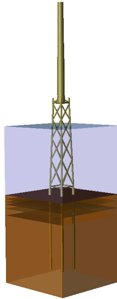
Fig. 2. 3D model of the jacket foundation.
