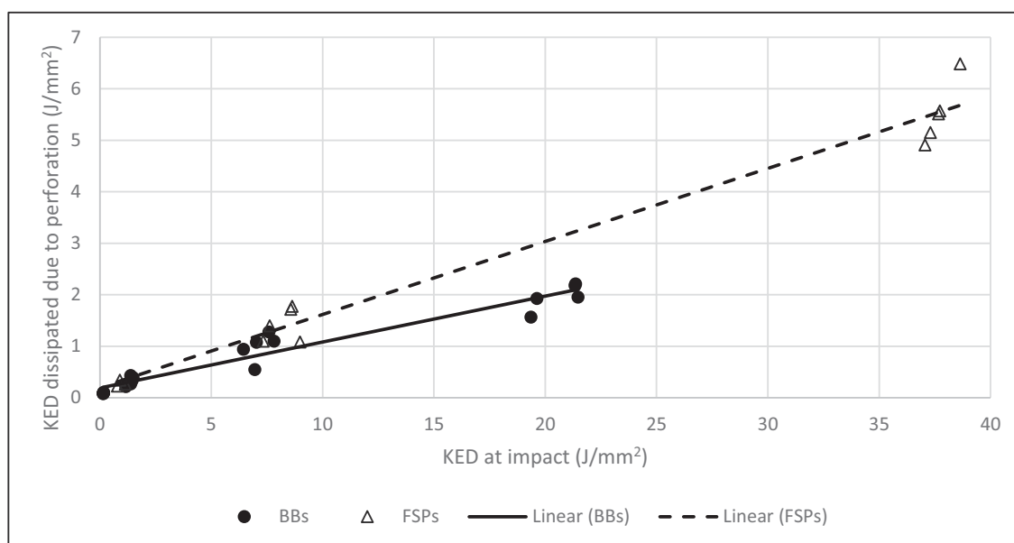
Fig. 5 Relationship between KED at impact and the KED dissipated due to perforating event for both FSPs
